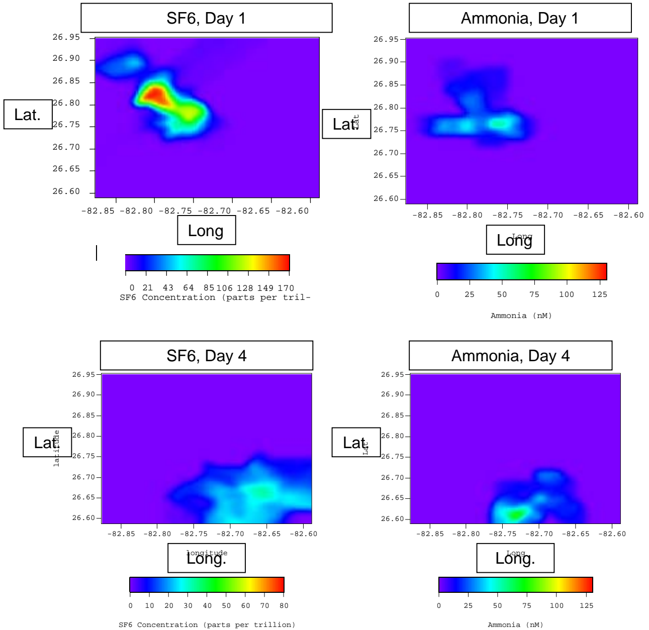
Figure 1: Time Course of Regions of High Ammonia and SF 6 on the W. Florida Shelf [Shows Color Contour Maps that Depict the Intermingling of West Florida Shelf Water Masses that are Enriched in Ammonia and Sulfur Hexafluoride and Fact that the Intermingling is Preserved as the Water Masses Drift to the Southwest for a Period of Four Days]
