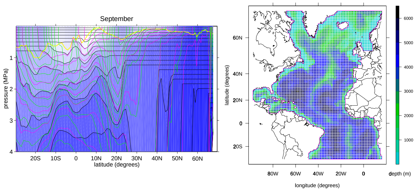
Figure 1 Left: Upper 400 meters along 31^\circ\text{W} for 1972 from the Atlantic 1.4^\circ HYCOM model without data assimilation. Shade of blue indicates potential density; black curves, interface pressure; magenta, potential temperature ( 2^\circ\text{C} spacing); green, salinity ( 0.2 psu spacing); yellow, bottom of the mixed layer. Right: Mercator projection of grid with map overlay and with colors indicating depth.
