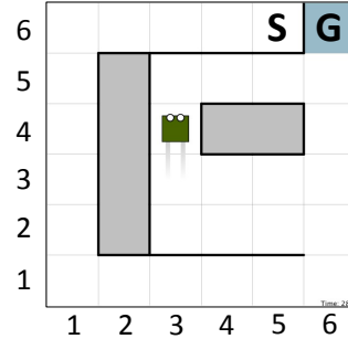
Figure 5. The baseline grid world task. To display the agent’s actions and state transitions to the trainer, (1) wheel tracks are drawn from the agent’s previously occupied cell, and (2) the simulated robot’s eyes point in the direction of the last action. The start and goal cells are labeled ‘S’ and ‘G’ respectively.
