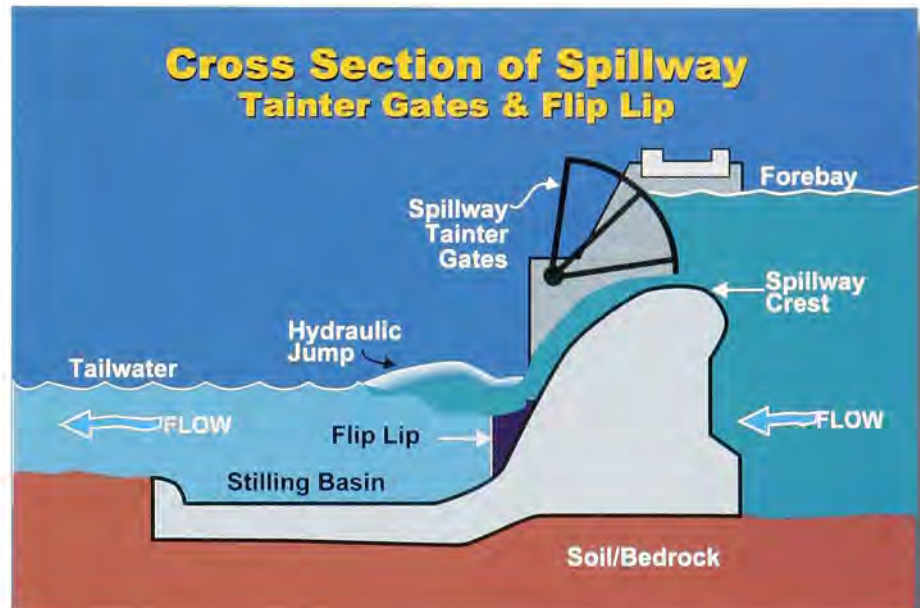
Flip Lip spill deflectors helped to move spill water in a more horizontal pattern to keep water from plunging deeply and to reduce the effects of gas supersaturation on fish.
