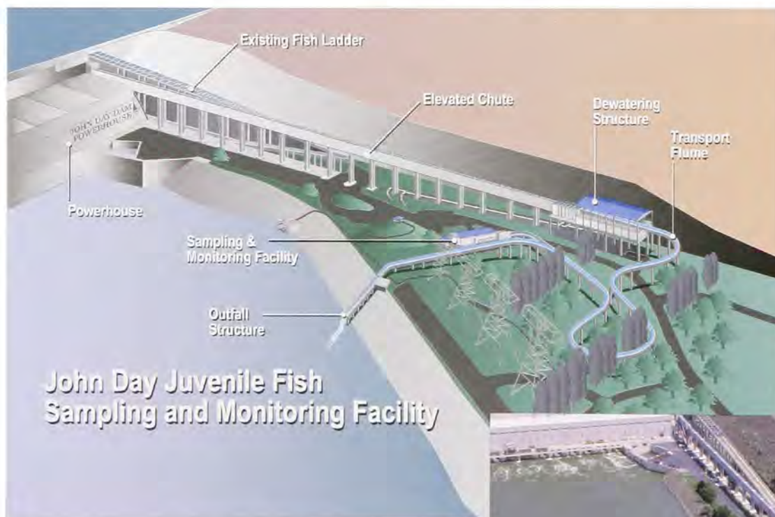
John Day juvenile fish monitoring and sampling facility.
