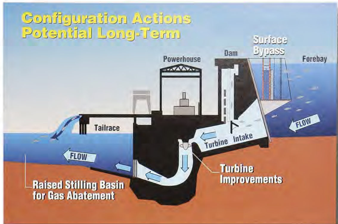
Potential long-term actions at the dams to benefit juvenile fish passage
