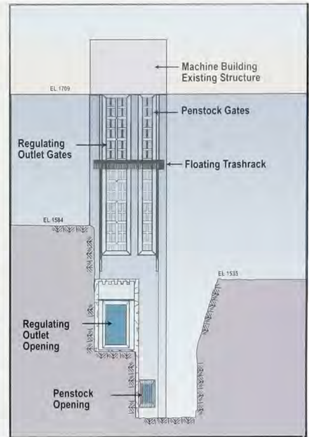
Modifications to the Cougar Dam temperature control tower began in 2002 with the drawdown of the reservoir. New outlet gates will be added to the tower to allow better water temperature regulation of water released from the reservoir.
