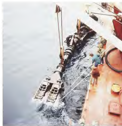
While the fishing ships corralled the oil, the dredge drag head was turned over to suction the oil swiftly into the hopper.
