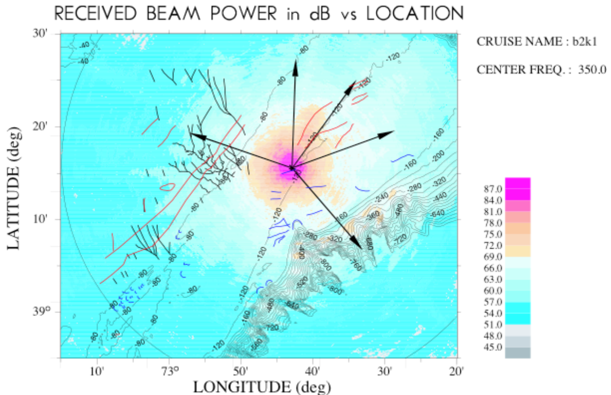
Fig. 1. Polar plot of the stacked (unambiguous) monostatic matched filtered reverberation on STRATAFORM from a SUS in a 50 Hz band centered at 350 Hz near Site S1. The black arrow directions indicates the 5 array headings, the base of the arrow the array position.
