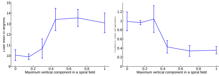
Figure 3.18: By varying the maximum z component in the spiral field we can control lobe amplitude and width.
