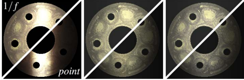
Figure 2.10: The clipping output is closer to the target (left) but loses global contrast. The cluster-based result (right) is darker in the red region enhancing the contrast. Visualized with our environment (top triangle) and point light (bottom). Generated with \alpha = 50 and 25 clusters.
