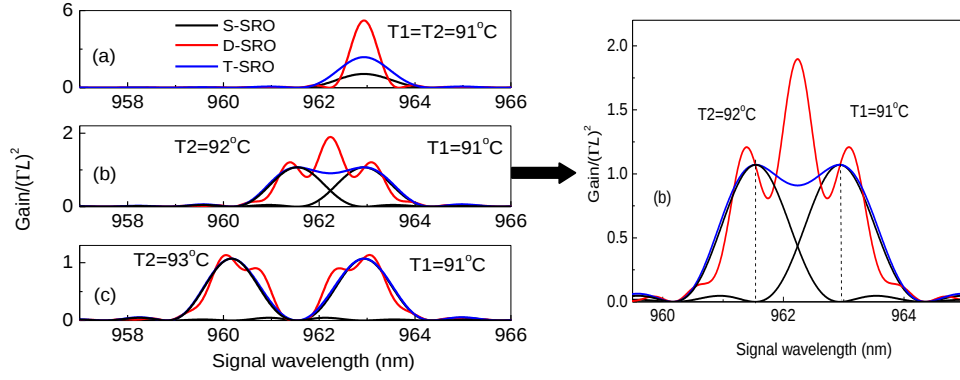
Fig. 3. Calculated gain of the S-SRO (black), D-SRO (red) and T-SRO (blue) versus signal wavelength at different combination of crystals' temperatures, (a) T_1=T_2=91^\circ\text{C} , (b) T_1=91^\circ\text{C} , T_2=92^\circ\text{C} and (c) T_1=91^\circ\text{C} , T_2=93^\circ\text{C} . Fig (b) is zoomed in the right side for further clarity.
