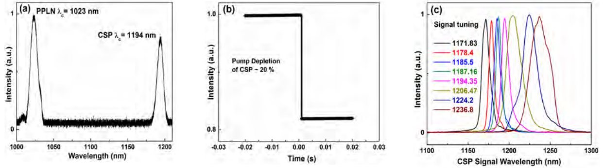
Fig. 2.2 (a) Simultaneous signal oscillation in MgO:PPLN and CSP OPO. (b) Pump depletion, and (c) Signal tuning and spectra with CSP OPO cavity delay.
