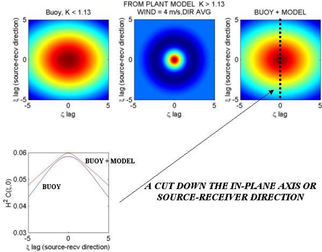
Figure 1. Upper left plot: Estimate of 2-dimensional sea surface roughness covariance function C(\zeta, \xi) made from directional wave buoy in the East China Sea during which wind speed was 4 m/s. This estimate is supported by wavenumbers K < 1.13 rad/m.
