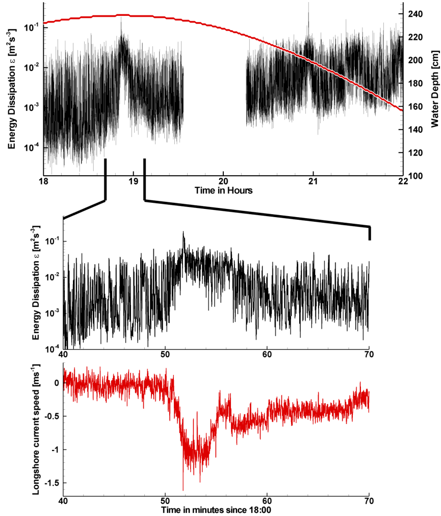
Figure 3. Upper Panel: Energy dissipation \varepsilon measured 0.5m from the bottom at 5Hz (black) and water depth at the sensor location (red) for a four hour period. Middle Panel: Expanded thirty minute period of \varepsilon showing the increased levels of turbulence between 50 and 60 minutes. Lower Panel: Longshore current speed from range averaged 2MHz Doppler measurements. Presumably these increased long-shore current speeds are associated with offshore-flowing rip-currents.
