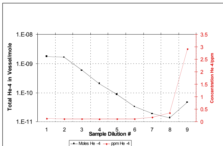
Figure 28. Evolution of He 4 moles in the vessel and He 4 concentration with the dilutions for the D 2 adsorption/desorption experiment on zeolite 13x.
