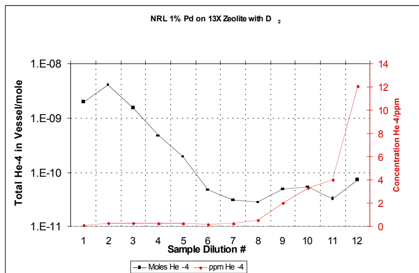
Figure 27. Evolution of He4 moles in the vessel and He4 concentration with the dilutions for the 2nd D 2 adsorption/desorption experiment on 1 wt% Pd/zeolite 13x.
