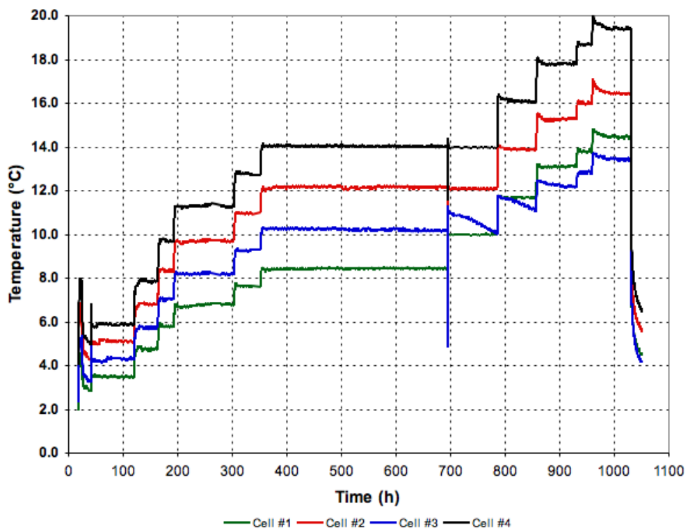
Figure 13. Temperature difference plot for the 4 matrix cell/calorimeters.
