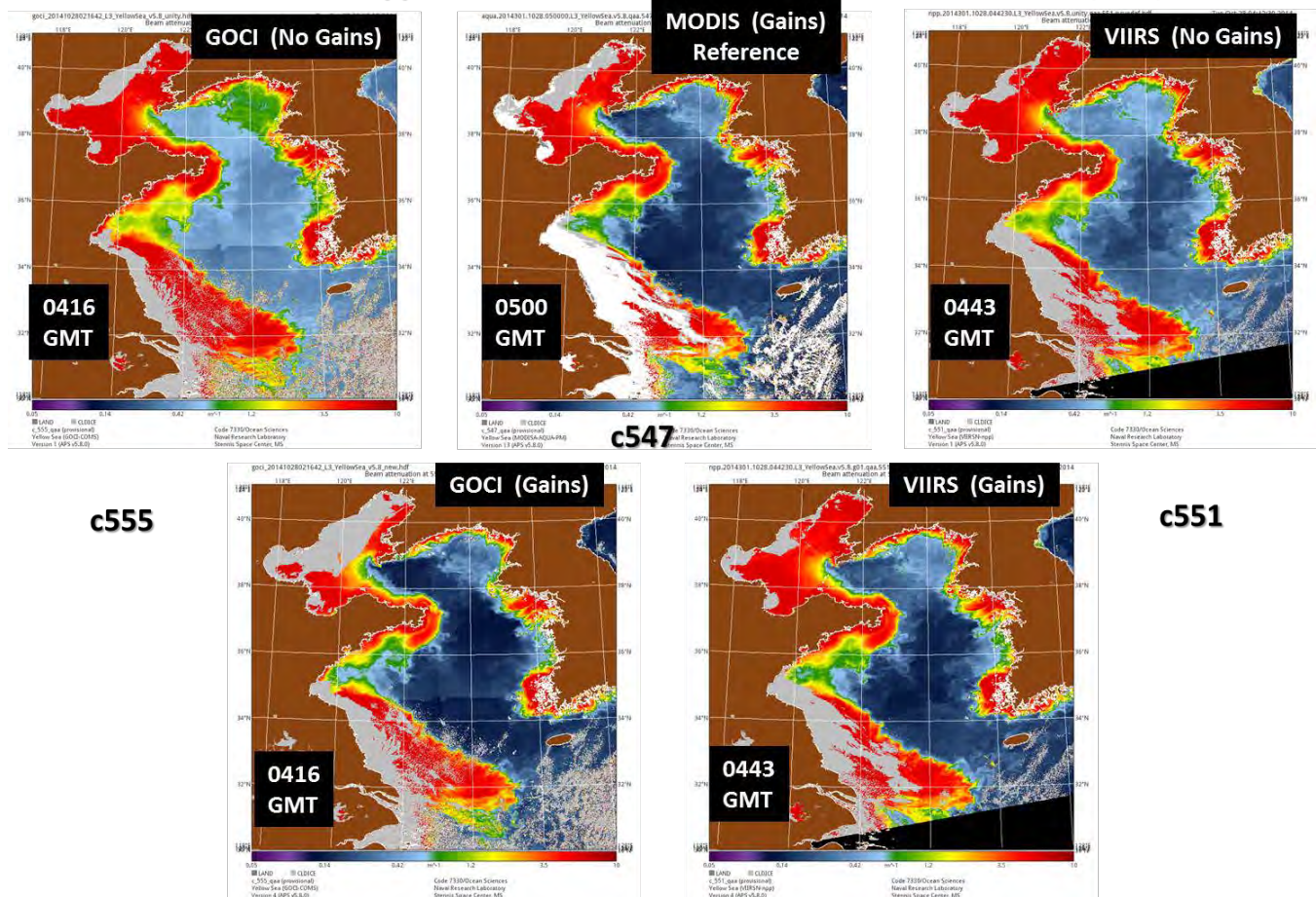
Figure 23 shows the GOCI, VIIRS and MODIS beam attenuation products in the Yellow Sea, October 28, 2014. The MODIS data, processed with appropriate calibration coefficients, represents truth (top center). The top left and right panels show the GOCI and VIIRS processed without vicarious calibration coefficients. The unity calibration for both sensors provides higher retrievals than the same day MODIS image. Bottom left and right images were created with AOPS v4.12 by applying the individual sensor gains from the corresponding tables in section 2. Both sensors show improved performance as compared to MODIS.
