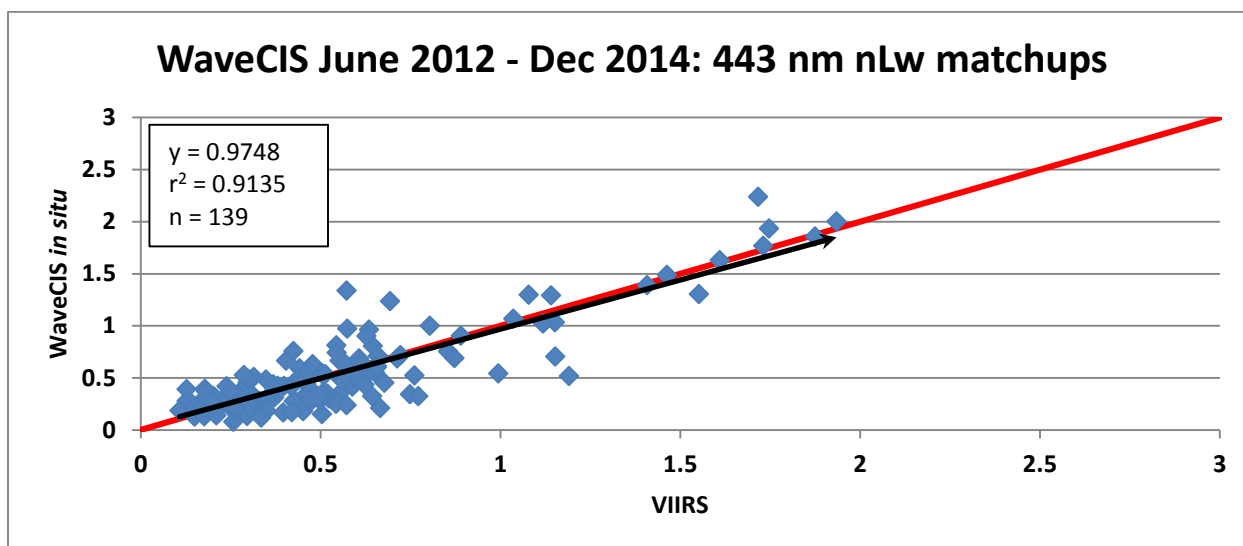
Figure 17 shows the 443 nm (M2) nLw matchups between the VIIRS satellite and in situ data from the WaveCIS site from 1 Jun 2012 up to 31 Dec 2014. Matchups are minimally screened, removing: negative values at any wavelength, extreme viewing angles, glint, clouds, navigation failures, atmospheric failures. A red 1:1 line is provided for reference. The regression and correlation coefficients indicate a tight correlation (close to 1) between the satellite and in situ sensors. Notice the correlation coefficient is lower than for the same channel than at MOBY ( r^2 = 0.9857 ). This is due to uncertainty from the complex marine atmosphere and dynamic (time/space variance) of the in water constituents.
