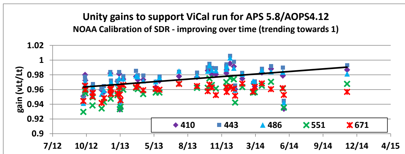
Figure 4 shows the VIIRS gain ( vLt/Lt ) over time at MOBY site using unity gain coefficients. In a perfect system in which all components are computed accurately, the vicarious TOA radiance ( vLt ) and satellite TOA radiance ( Lt ) should have a ratio of 1.0. Most of the ratios are below the 1.0 line suggesting the sensor without vicarious calibration is slightly high. The mean gain set for the 412, 442, 490, 555, and 668 channels were determined to be 0.9711, 0.9769, 0.9729, 0.9564, and 0.9587 respectively. The data also show the satellite continues to require periodic calibration updates as a stable system would exhibit no trend.
