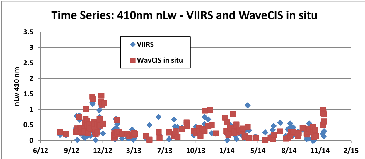
Figure 15 shows the time series for the VIIRS M1 (410 nm) channel plotted with the in situ value taken at WaveCIS. The satellite generally captures the trend of nLw at this station over the time period. The satellite data ( n = 139 ) is only screened for atmospheric and navigation failures, high satellite angles, and glint, therefore outliers are expected. Less stringent screening was intentionally employed to provide more of an operational description of the data.
