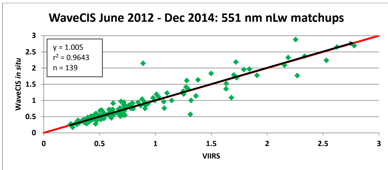
Figure 19 shows the 551 nm (M4) nLw matchups between the VIIRS satellite and in situ data from the WaveCIS site from 1 Jun 2012 up to 31 Dec 2014. Matchups are minimally screened, removing: negative values at any wavelength, extreme viewing angles, glint, clouds, navigation failures, atmospheric failures. A red 1:1 line is provided for reference. The regression and correlation coefficients indicate a tight correlation (close to 1) between the satellite and in situ sensors. Notice the range of VIIRS (0.23 – 2.8) more appropriately covers the natural range of nLw from open ocean to coastal waters, compare to MOBY (0.15, 0.5) . This is due to stronger reflectance of green light in the coastal waters, effectively increases signal to noise ratio .
