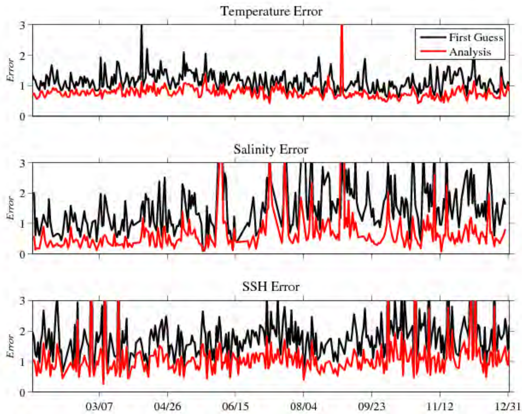
Figure 3-6. Errors in temperature (top), salinity (middle), and SSH (bottom) solutions from the first guess (black) and the analysis (red) relative to the observations that were assimilated for the 4DVAR SSH experiment, which assimilated SSH directly. These errors span the entire year of the Okinawa Trough experiment (15 January through 31 December 2007) and are normalized by the corresponding observation error (Equation 5).
