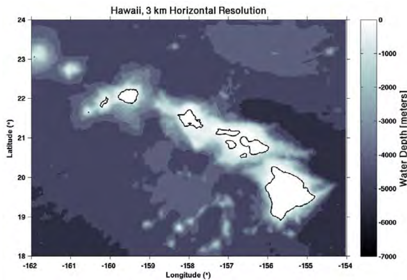
Figure 4-13. Test Case 4: RIMPAC model domain of the Pacific Rim of Hawaii at 3 km resolution. Water depth is in meters. The domain is located at 18°N to 24°N and 162°W to 154°W, with a horizontal resolution of approximately 3 km.
