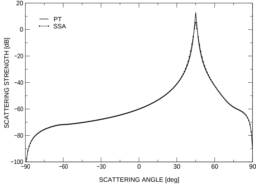
Figure 1: Bistatic scattering strengths as a function of scattering angle for lowest-order PT and SSA for h = 0.1 m, l = 10 m, f = 3 kHz, and an incident angle of 45^\circ ( k_w h = 1.26 , k_w l = 125.66 ). The PT and SSA results agree over the entire range of scattering angles except in a very narrow angular region around the specular direction. This indicates that for this problem the PT results are accurate.
