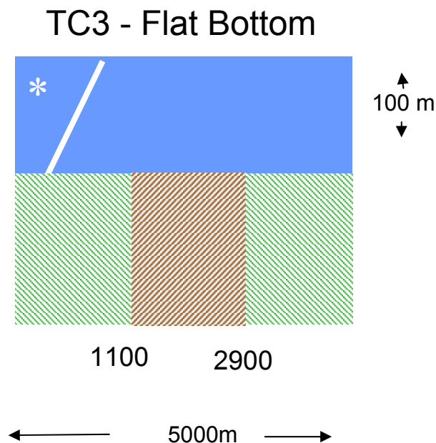
Figure 3. Geoacoustic environment for test case 3.
