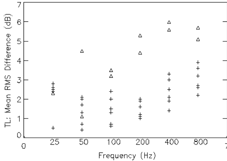
Figure 4. Mean RMS differences between transmission loss (TL) calculated for the estimated profiles and the actual profile, for a source and receiver depths of 80 m.
