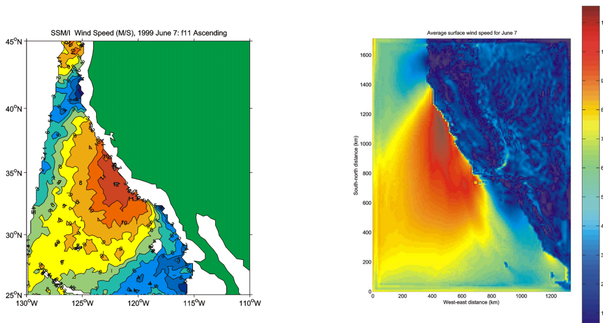
Figure 2. Surface wind speed on 7 June 1999 as derived from the SSMI satellite data (left panel) and predicted with the MM5 atmospheric model (right panel).
