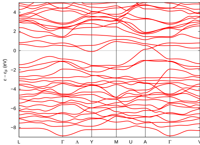
FIG. 11. (Color online) The electronic band structure for structure #35, one of our approximations to the “ r - W_2N_3 ” structure [21], using the PBE functional.
