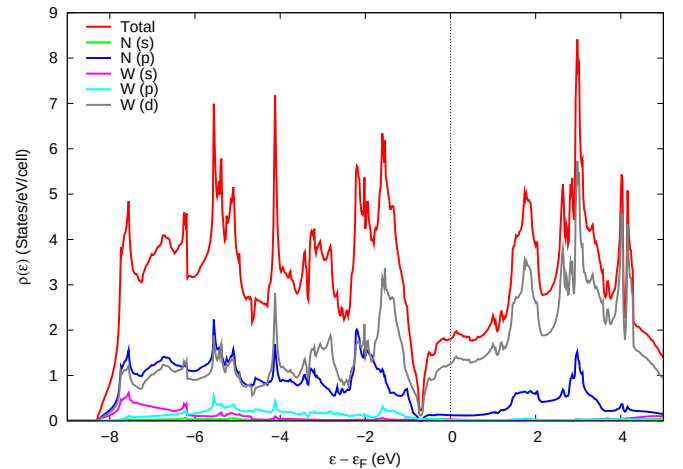
FIG. 7. (Color online) The electronic density of states and angular momentum decomposed density of states for tungsten nitride in the NbO structure (#53). These were computed via the tetrahedron method in VASP. The primary contributions are from the N- p and W- d states, with the W- d states dominating the conduction band.
