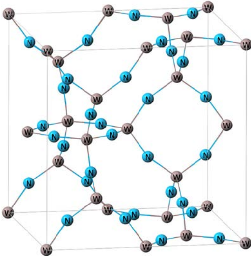
FIG. 13. (Color online) The SiO_2 -like cI36 structure (#15 in the Supplemental Material [48]) predicted as the ground state of N_2W by the vdW-DF2 functional. The basic structure looks the same using LDA, PBE, and vdW-DF2 functionals. The exact dimensions are described in Table VI. Note that this is a body-centered-cubic lattice, so the center of the cube and the cube corners are equivalent sites. The inversion sites are at the centers of the eight-atom rings, not on the tungsten atoms.
