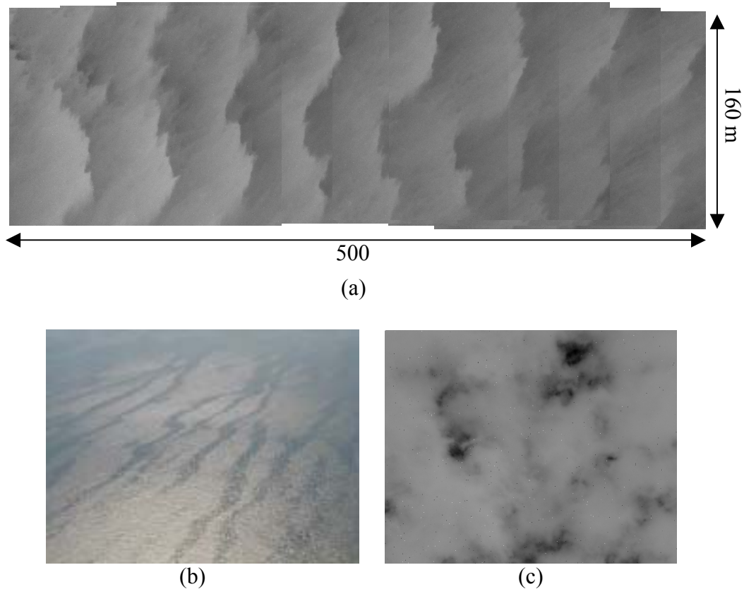
Figure 4. Mosaic of infrared images (a) showing the successive fronts of ocean skin temperature in the presence of ubiquitous surface slicks observed on 8-22-02 during a period when the wind was 5 m s -1 from the SW. The top of the mosaic is East. (b) Picture of the ocean surface slicks observed on the ocean surface during the overpass that produced the mosaic in (a). (c) Infrared image of the sky showing that the ocean surface features observed in the downward looking imagery in (a) are, in fact, real temperature structures.
