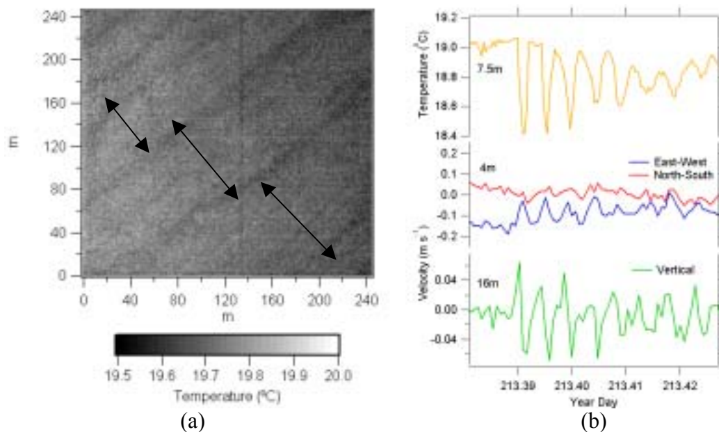
Figure 2. (a) Example of fine-scale infrared imagery as observed from the aircraft showing banding features observed during the passage internal waves through the CBLAST-LOW site south of Martha's Vineyard for low wind speed conditions (4 to 6 m s -1 ) taken on 8-1-01 (North is up). The arrows highlight the spacing between dark bands corresponding to cooler temperature. The spatial scale of the banding features ranges from 50 to 100m. (b) Temperature and velocity time series measured at the SECNAV buoy site showing the structure evident of the passage of internal waves.
