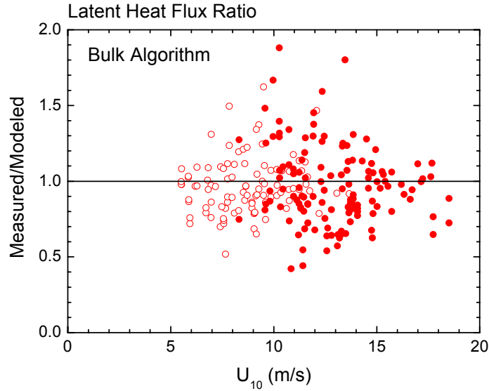
Figure 2. As in Fig. 1 except this shows the latent heat flux ratio. Filled circles denote cases when the modeled spray flux ( Q_{L,sp} ) is at least 10% of the modeled interfacial flux ( H_L ). The average of the ratios in this figure is 1.010, and their correlation coefficient with wind speed is 0.066.
