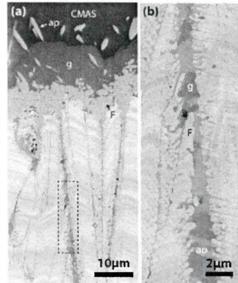
Figure 7: CMAS infiltration into intercolumnar gaps in the EB-PVD YbZO coating. The large garnet grains at coating surface in (a) are similar to those observed in the pellet-based tests. The limited volume of apatite formed in the gaps (b) does not efficiently block penetration.
