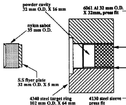
Fig. 1. Target fixture and flyer plate assembly used in the shock consolidation. Note that only the sample, and not the containment assembly, is impacted.
