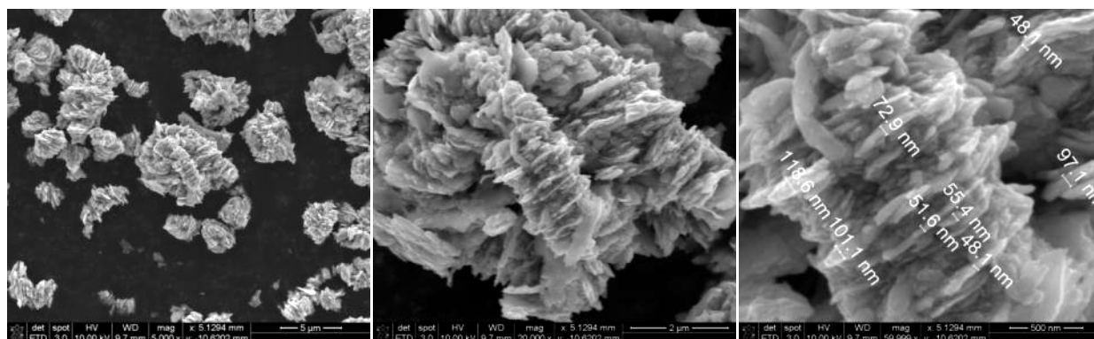
Figure 4.10. Sample 3-4a ( \text{SmCo}_5 , Valeric acid, Milling time: 8h)
