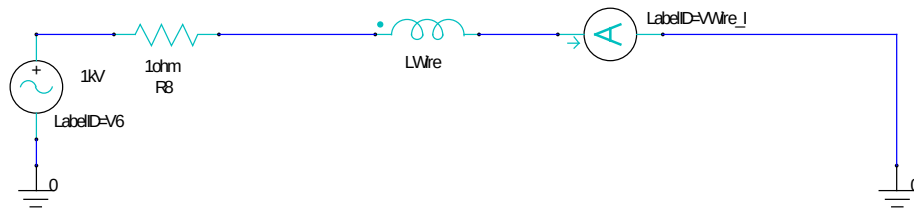
Figure 4.63. Corresponding electrical circuit schematics
