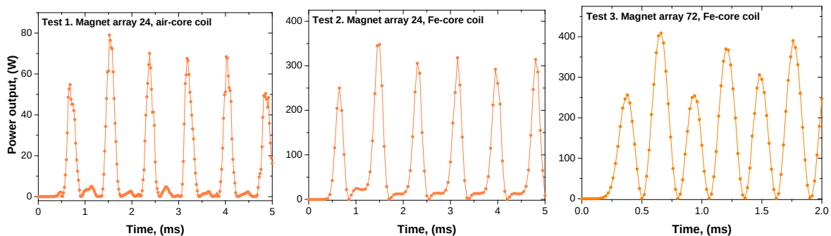
Figure 4.53. Power Output Data
