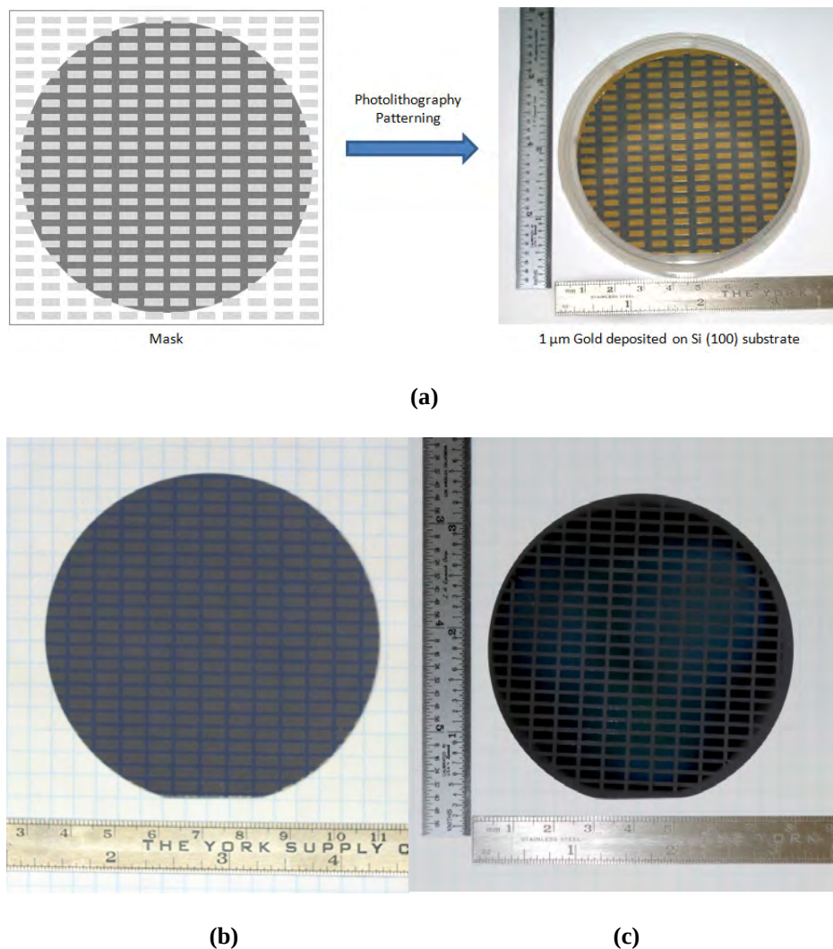
Figure 3.20. (a) Post-deposition processing via standard photolithography techniques (negative resist NR71-3000) followed by 1 μm Au sputtering and removal of Au with RR41 photoresist remover to generate discreet composition units in the calibration sample. The same process was followed for the (b) Ni standard sample and the (c) \text{Ca}_3(\text{Fe,Ni,Co})_4\text{O}_9 combinatorial ternary sample (with HCl etchant).
