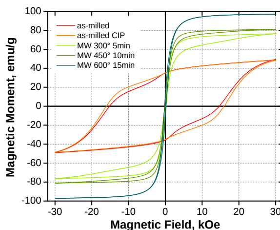
Figure 4.29. Magnetic hysteresis data for as-milled and microwave sintered nano-scale \text{SmCo}_5
