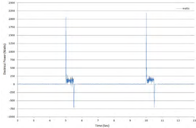
Figure 6.7. DC Bus Electrical Power in Step Response Test
