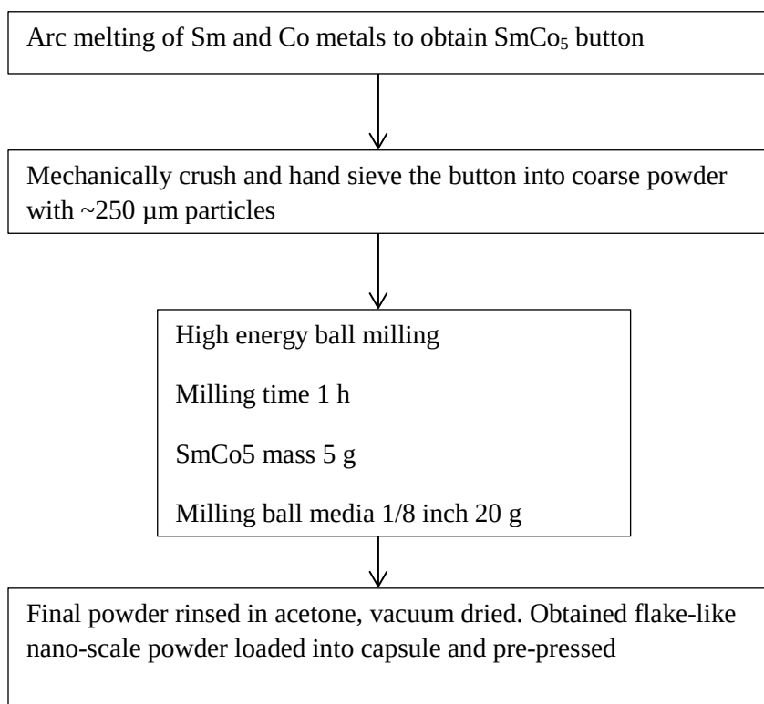
Figure 4.20. \text{SmCo}_5 experimental powder preparation flowchart
