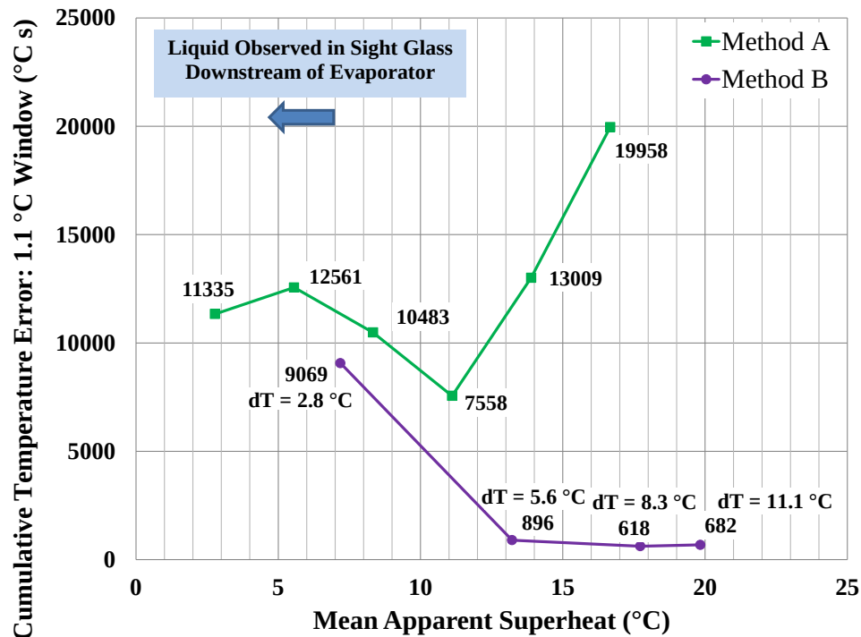
Figure 1.14. Temperature error summary
