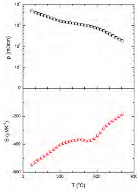
Figure 3.29. Temperature dependence of electrical resistivity \rho (top) and Seebeck coefficient S (bottom) for CMO bulk sample
