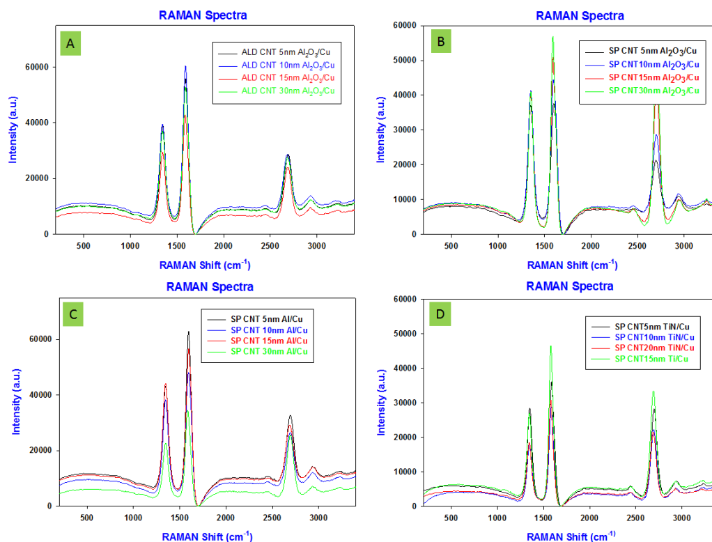
Figure 5.7. Raman Spectroscopy of the CNT/Cu sample b (FCCVD)
