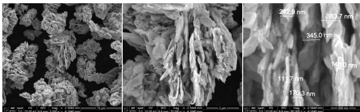
Figure 4.9. Sample 3-1a ( \text{SmCo}_5 , Valeric acid, Milling time: 4h)
