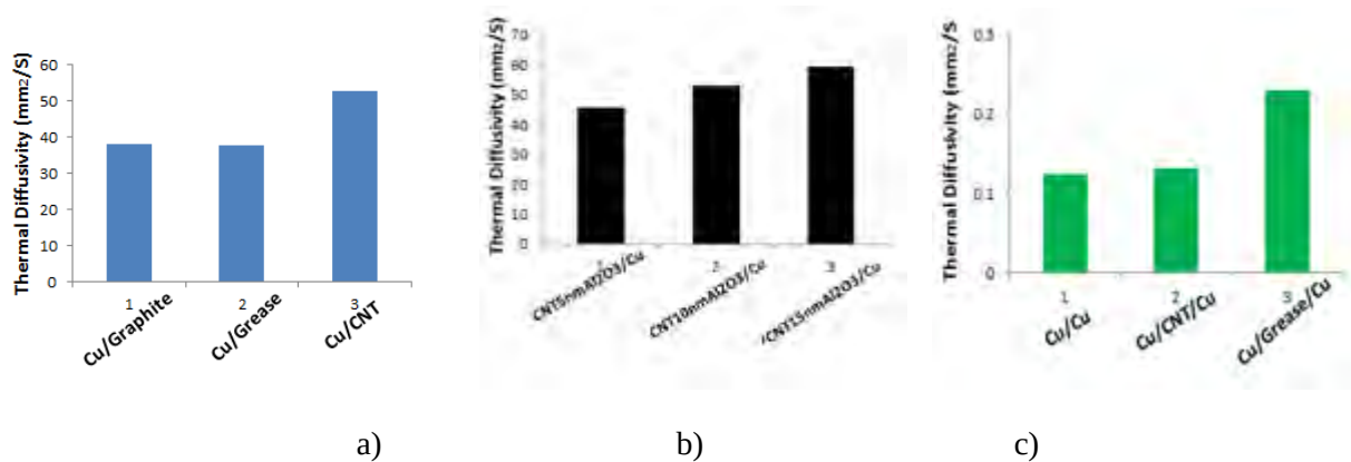
Figure 5.10. LFA results -Thermal diffusivity of various samples a) The effect of different coating materials on thermal diffusivity b) The effect of CNT density and length on thermal diffusivity c) The effect of different interface materials on thermal diffusivity
