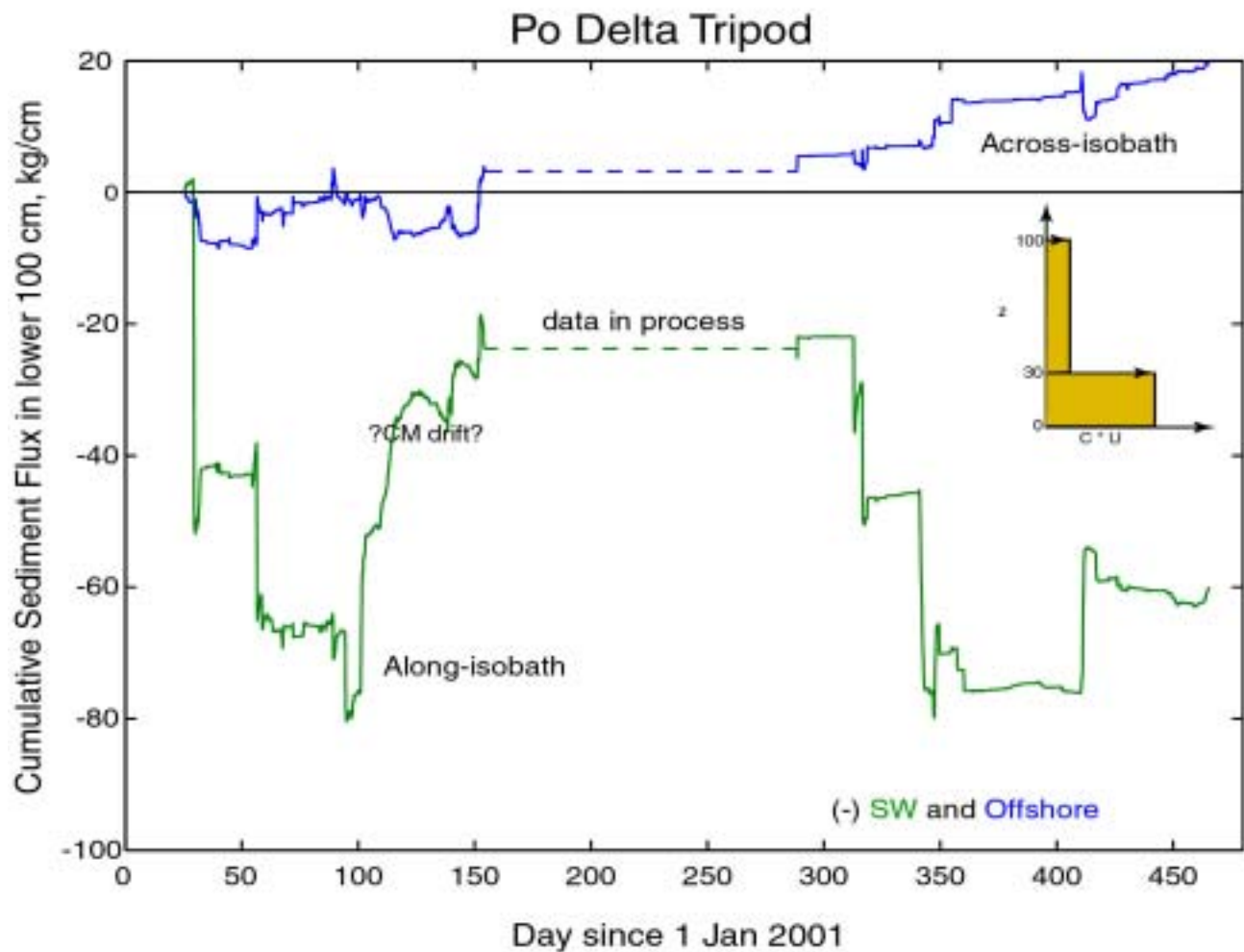
Figure 1. Cumulative sediment flux for the 15-mo record on the Po River delta. The net flux over this period is dominantly to the SW and slightly offshore. The large Bora wind events appear to drive the net sediment flux in the alongshelf direction with the smaller Scirocco events having less impact.
