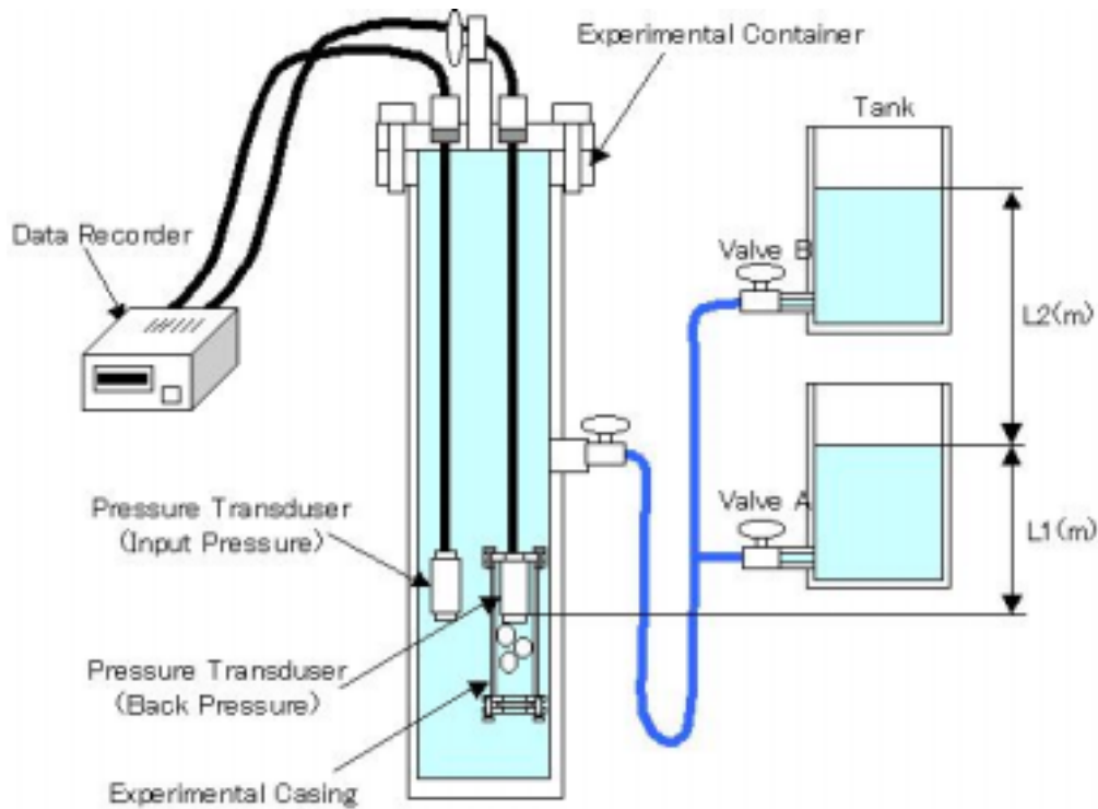
Figure 2 Experimental Container in which the Damping and the Phase Shift of Back Pressure from Input Pressure were examined for several samples to select the suitable filter.
