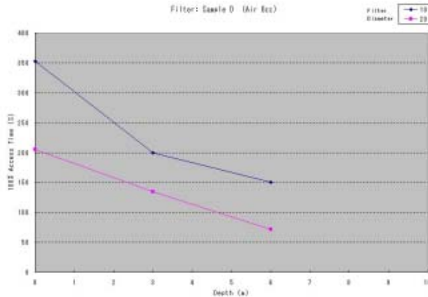
Figure 3 The Access Time of Back Pressure to 100 % of Input Pressure Reduce with the Water Head (Depth of Water).
