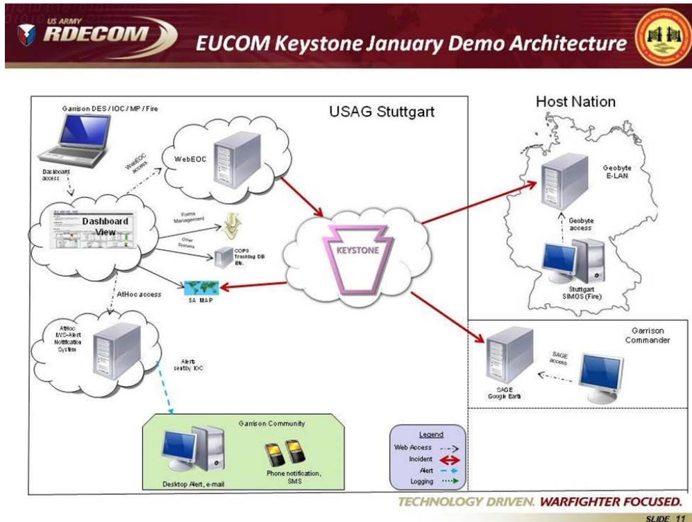
Figure 5: EUCOM Keystone CONOPS Demonstration Architecture
