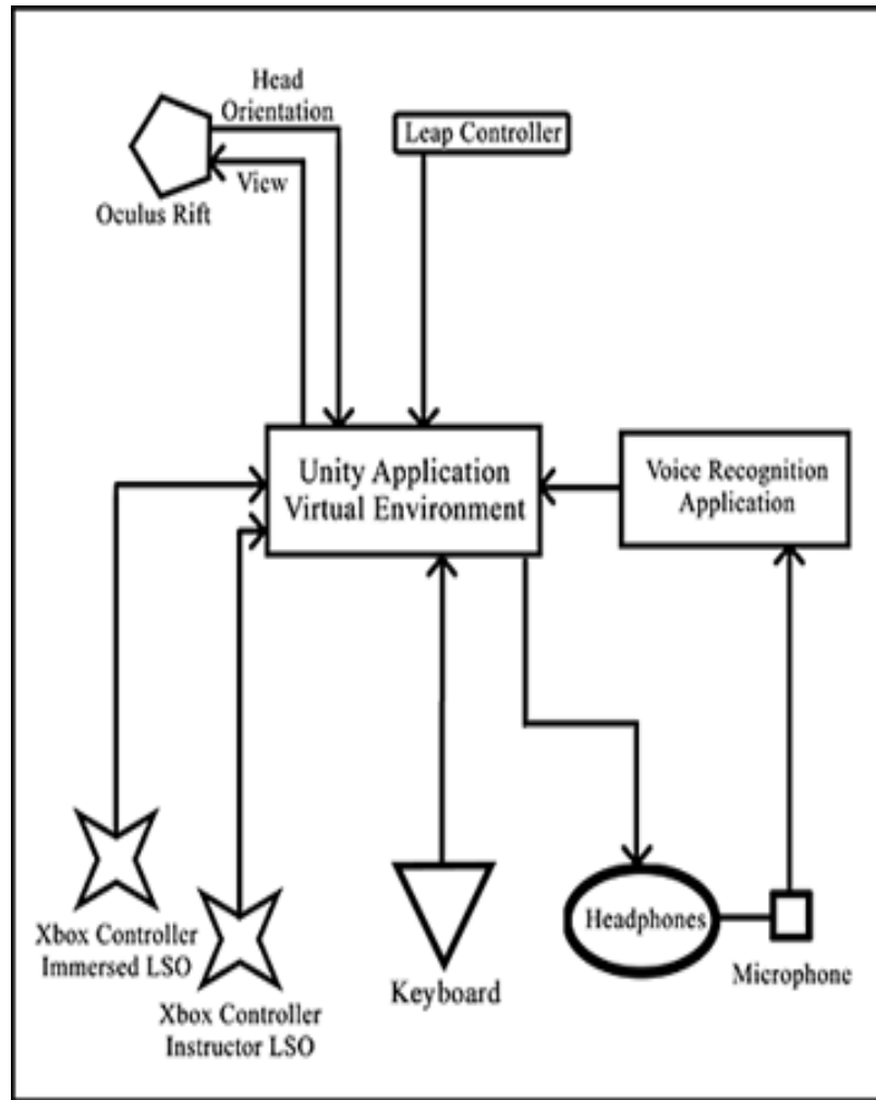
Figure 20. Hardware/Software Architecture
