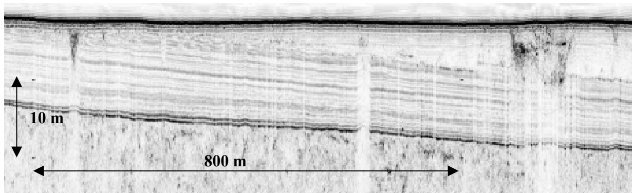
Figure 1 Chirp subbottom profile collected in phase 1 survey area in 80 meters of water off New Jersey coast . The image was generated using a 40 msec 1.5-4 kHz FM pulse. The image shows potential causes of geoclutter including buried river channels and gassy sediments indicated by acoustic whiteouts and early arrival times of reflections under the gassy features.
