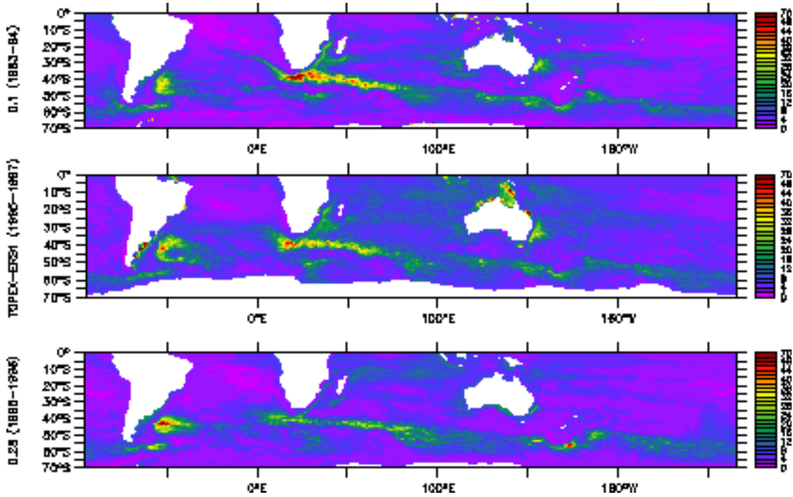
Figure 1. Sea Surface Height variability (in cm) for the Southern Ocean from the 0.1^\circ global simulation (top), blended TOPEX-ERS1 satellite data (middle), and the 0.28^\circ global simulation (bottom). [Color plots show up to 70+ cm of variability in eddy-active regions, such as the Agulhas Retroflection and the Brazil-Malvinas Confluence.]
