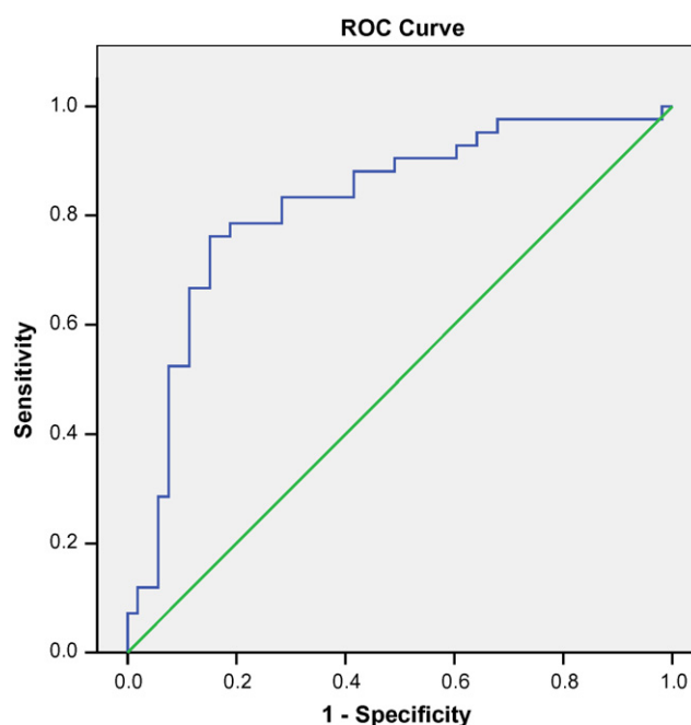
Fig. 4 – ROC Curve using %TBSA burn injury and survival time after burn to predict the presence of fungal elements during autopsy. Area 0.823 ( p < 0.01 ).
