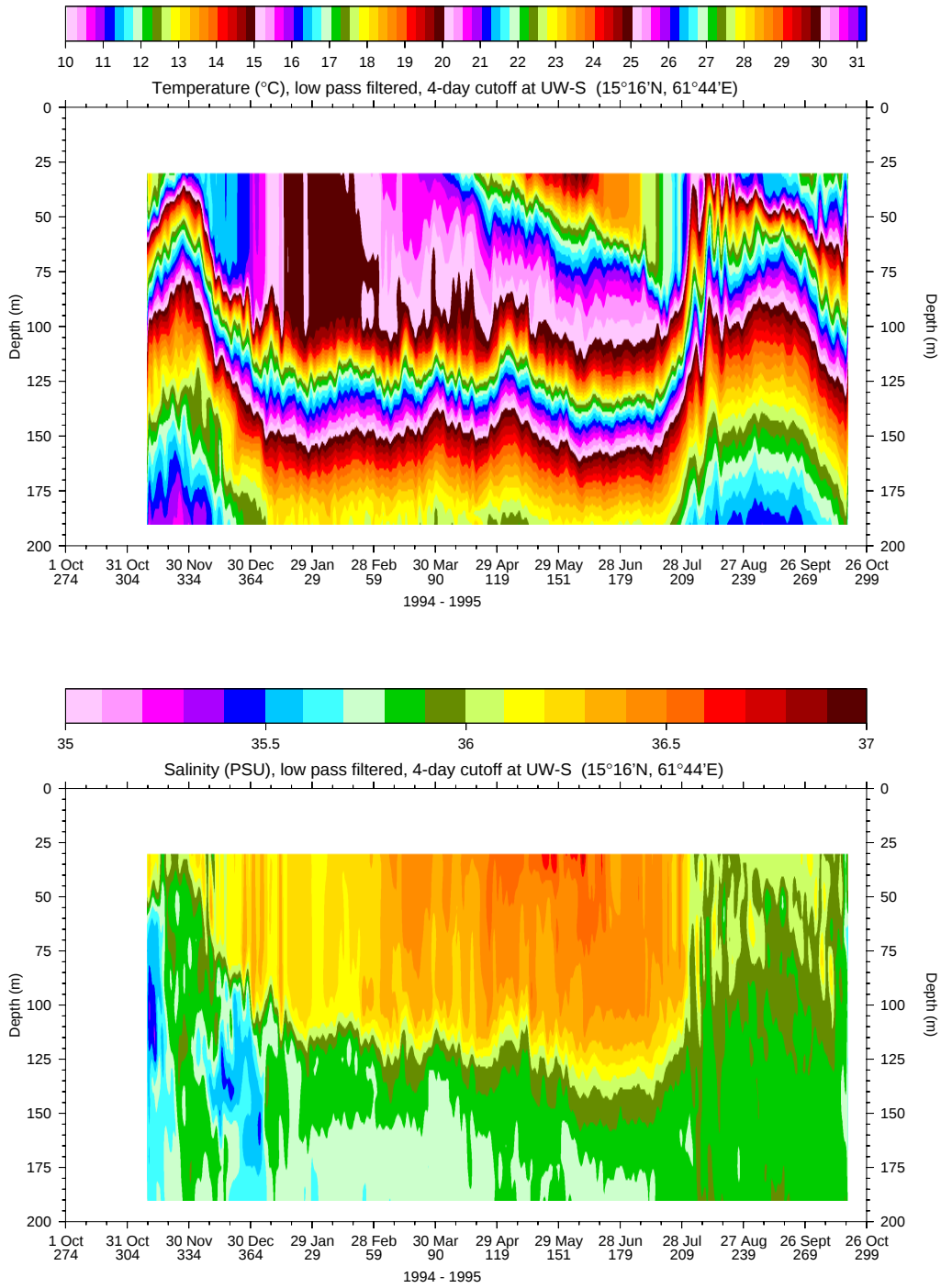
Figure 1. Four-day low pass filtered temperature (upper) and salinity (lower) from site UW-S in the Arabian Sea. The contour intervals for temperature ( 0.25^{\circ}\text{C} ) and salinity ( 0.1\text{PSU} ) are approximately equal in their contribution to density ( \sim 0.075\text{ kg/m}^3 ). The temperature color scale repeats every 5^{\circ}\text{C}
