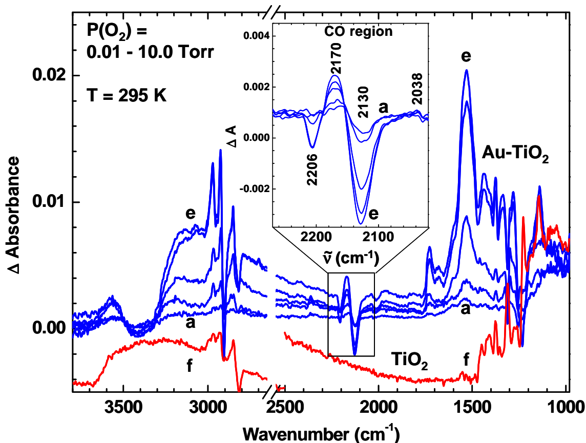
Figure 1.8: Difference spectra showing the evolution of Au + (2170 cm -1 ) and the depletion of Au δ+ (2130 cm -1 ) by monitoring \nu_{co} . 17
