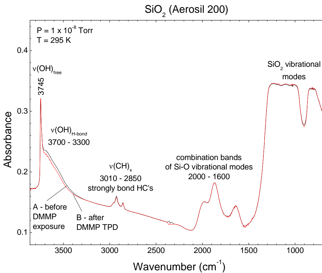
Figure 3.4: Infrared spectrum of silica before DMMP exposure (A) and after temperature programmed desorption of DMMP (B), showing a minimal change in absorbance after thermal desorption of the adsorbed species.
