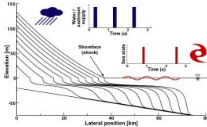
Figure 1. Moving-boundary, morphodynamic model of constructional shelf clinoforms illustrating the characteristic-event (flood and storm) approach.
