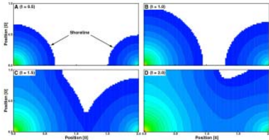
Figure 2. The interference of two fluvio-deltaic systems over the time interval 0 < t < 2 . Sediment / water point sources are located in the lower left and right corners of each panel; the sediment source in the left corner is twice as large as that in the right. Only the subaerial (fluvial) elevation is contoured. Warmer colors indicate higher elevations; ocean surface is white.
