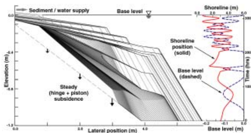
Figure 4. Predicted strata and shoreline position for the recent physical experiment on continental-margin response to sea level in the XES basin at SAFL.
