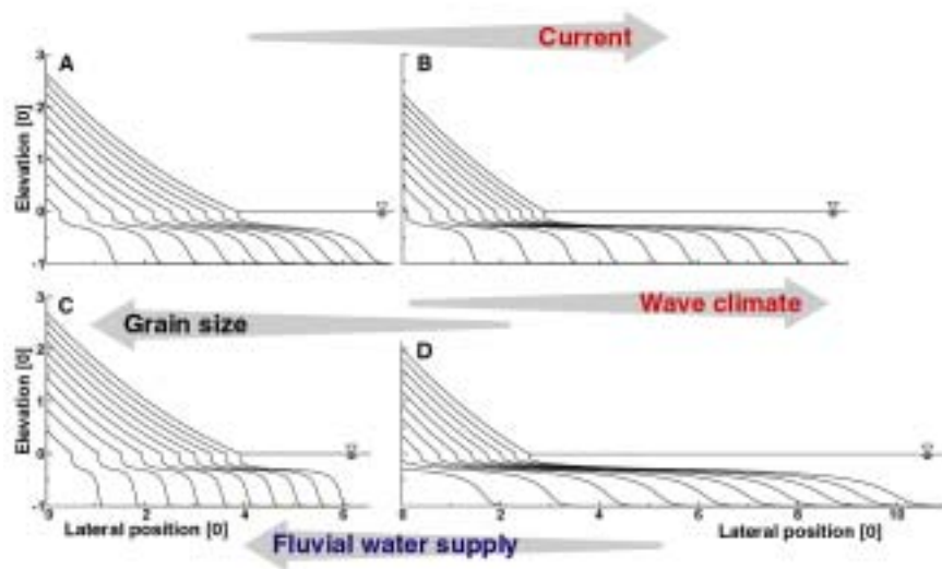
Figure 3. Morphology of shelf clinoforms as a function of grain size, wave and current climate, and fluvial water supply.
