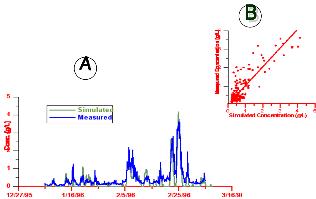
Fig. 2. Calibration to suspended sediment data. A: Comparison of simulated suspended sediment concentrations with measurements from the VIMS tripod at 15 cm above the sea floor. B: Correlation plot or C > 0.2 g/l
