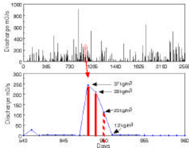
Figure shows the first 7-yr of a 1000-yr daily discharge (HydroTrend) simulation of the Chienti River, Italy. The annual discharge is \approx 10 \text{ m}^3/\text{s} . Seasonal floods that last for 1 to 3 d can exceed 500 \text{ m}^3/\text{s} . The lower panel shows a 3-d flood event with discharges in the 100 - 250 \text{ m}^3/\text{s} range and sediment concentrations in the 20 - 37 \text{ kg/m}^3 range. The river would likely go hyperpycnal for the first two days of the flood.
