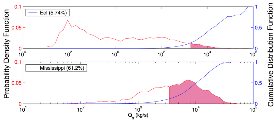
Figure shows the probability density function of the sediment load for the Eel River, California, and the Mississippi River, along with their cumulative distribution function. In the Eel case, 5.74% of the days moves 90% of the sediment. In the Mississippi case, 61.2% of the days are needed to move 90% of its annual sediment load.
