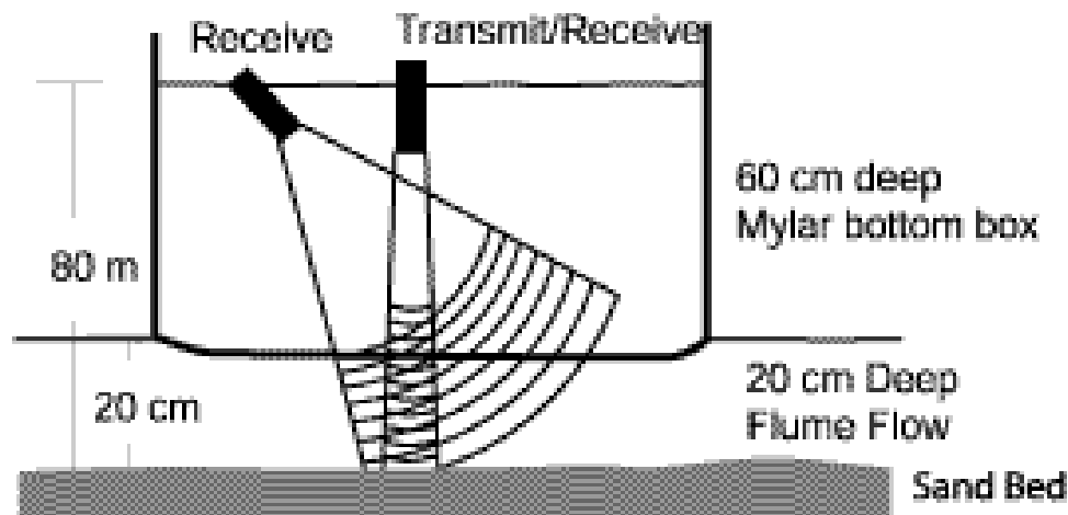
Figure 1. The bi-static geometry used in the flume test allows resolution of both bedload and suspended load fluxes. Due to the 20 cm depth of the flume an acoustically transparent bottom box was installed above the flume to house the transducers in a “field” geometry
