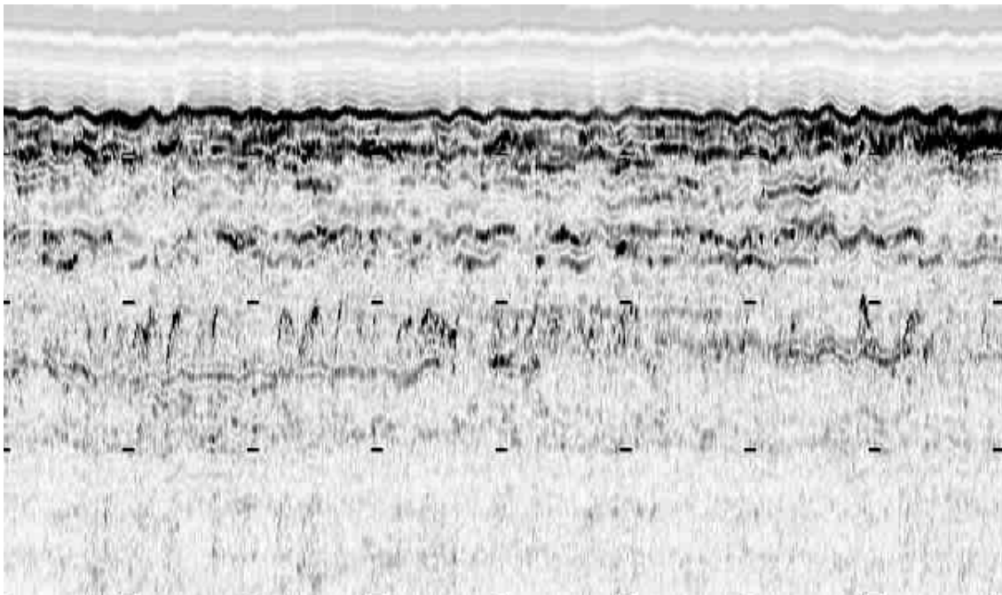
Figure 1. Chirp sonar profile of sediment at Corpus Christi mine burial site generated in November 2001. Note that the sediments are neither vertically nor horizontally homogeneous. The complex sediment structure is most likely due to storm driven erosional processes. Note that seafloor oscillations in the image are caused by gravity waves causing pressure fluctuations at the sonar vehicle which was towed 5 meters above the seabed. The ticks in the image have a vertical separation of 5 meters. The top of the image is 15 meters from the sea surface. The bottom of the image is 35 meters from the sea surface
