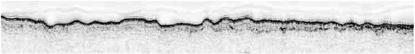
Figure2. Chirp sonar profile of sand seabed at Martha's Vineyard mine burial site generated in August 2002. Note that the sediments are homogeneous with the exception that a weak reflector sometimes appears within a meter of the sediment-water interface. The water depth is 15 meters. The vertical width of the image is 4 meters
