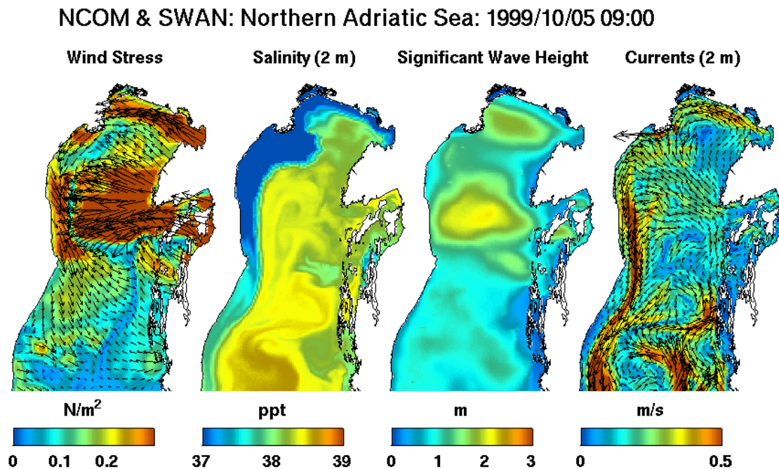
Figure 2: Snapshot of circulation and wave calculations for realistic simulation of October, 1999 showing (a) wind stress magnitude and direction from COAMPS™, (b) salinity, (c) SWAN-predicted wave height, (d) near-surface current magnitude and direction. Figure illustrates the complex nature of wind, wave, and currents in the Northern Adriatic; provided courtesy of Rich Signell, SACLANT-CEN.
