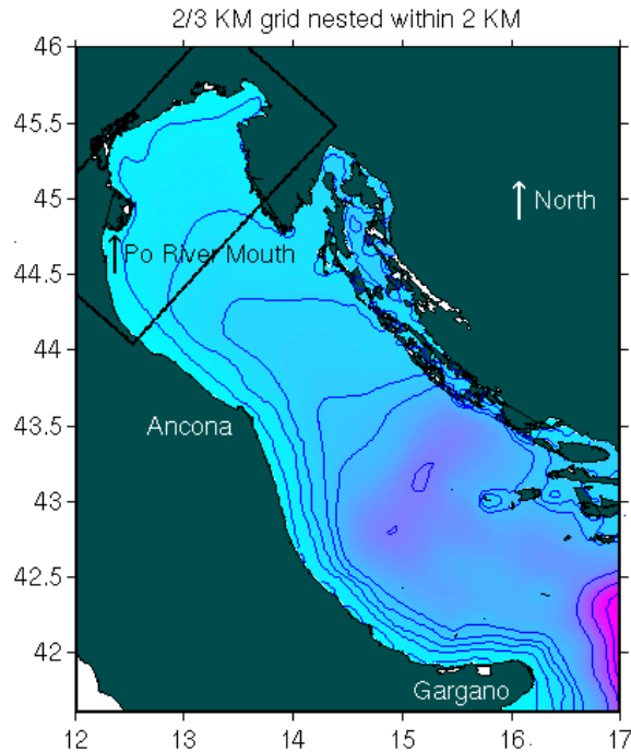
Figure 1: Northwestern Adriatic Sea, showing location of Po River mouth; bathymetry indicated by color and contour lines (every 20m). The location of the high-resolution nested model grid (2/3 km grid) outlined by the box in the northwestern Adriatic.
