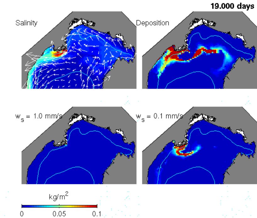
Figure 3: Estimates of (a) surface circulation and salinity; (b) sediment deposition; and depth-integrated amount in suspension for sediment modeled as (c) flocculated; w_s=1.0 mm/s; and (d) unflocculated, w_s=0.1 mm/s. Calculations made on 2 km grid at day 19 of the January, 2001 simulation using COAMPS™ wind field and concurrent record of daily Po River discharge from Pontelagascuro; but neglecting waves.
