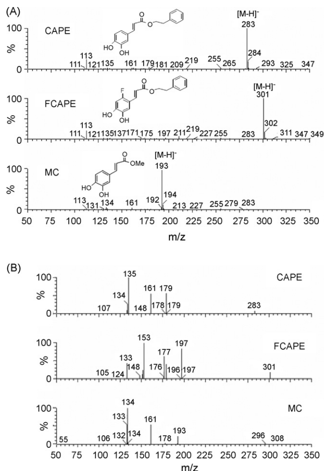
Fig. 1. Full scan mass spectra for CAPE, FCAPE, and MC (A) and product ion mass spectra where product ions m/z 135, m/z 153, and m/z 134 were monitored for CAPE, FCAPE, and MC, respectively (B). The collision energy for the MS/MS is 20 V.
