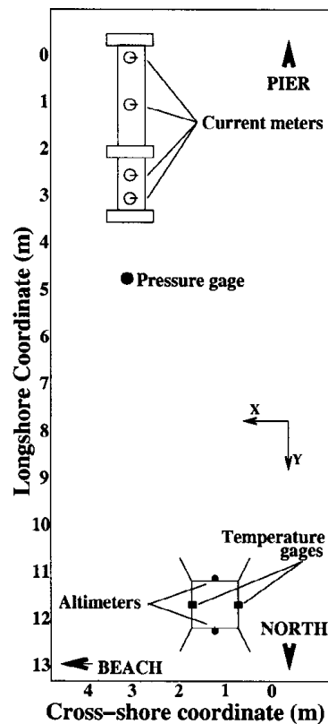
Figure 1. Plan view of bottom-stress and megaripple detection instrument array. The four acoustic Doppler current meters (ADVs) (SonTek “Ocean” probes) were deployed in an alongshore array in approximately 4.5-m water depth, about 60 m north of the Scripps pier, La Jolla, CA. The acoustic altimeters provide estimates of seafloor elevation, and the pressure gage (buried to reduce flow noise) measures bottom pressure, which can be converted to sea-surface elevation using linear wave theory. The temperature measurements were used to estimate the squared buoyancy frequency to determine stratification. [sketch: Neighboring near-bottom current meters are separated 0.5, 1.0, and 1.5 m alongshore. Two altimeters and 2 temperature sensors are deployed about 75 cm above the seafloor 10 m alongshore of the current meters. A pressure gage was deployed between the current meters and the altimeters.]
