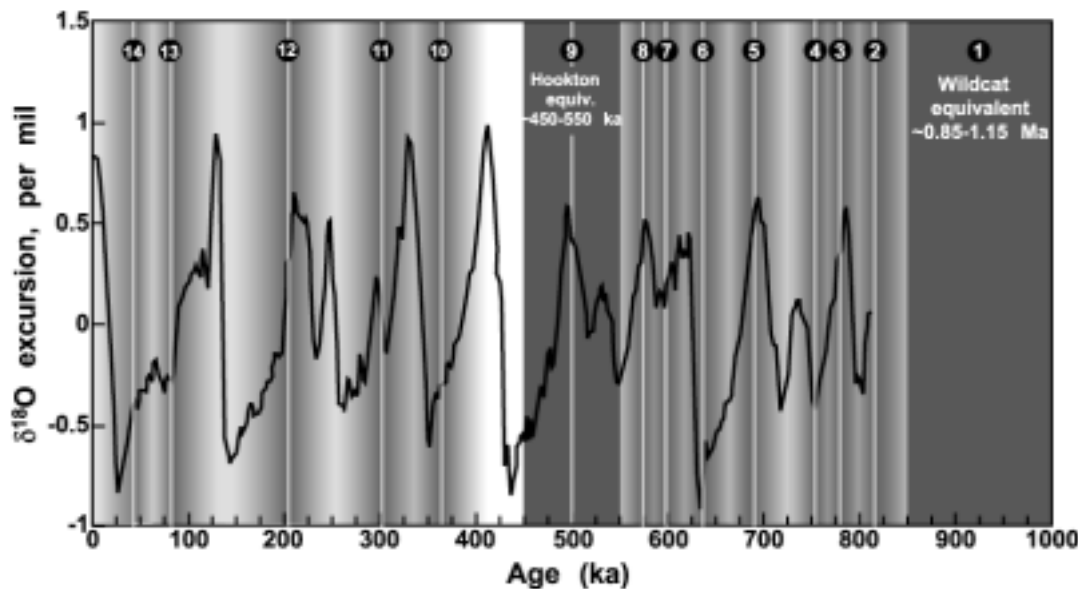
Figure 1 – Stacked \delta^{18}\text{O} curve derived from fourteen different benthic records globally (Medeiros et al., 2000). Vertical lines show estimated ages of Eel River Basin seismic unconformities; shading represents uncertainty in our age estimates. Solid gray areas represent estimated hiatus durations of the "Hookton" and "Wildcat" equivalents (Surfaces 1 and 9). Note the increased frequency of unconformity formation prior to ~550 ka, mimicking the obliquity-dominated 41 kyr glacioeustatic cycles during that same interval. After the Hookton Datum hiatus, the frequency of unconformity formation decreases, and coincides with the eccentricity-dominated 100 kyr cycles during that interval. The apparent correspondence between \delta^{18}\text{O} cyclicity and unconformity formation both before and after the orbitally-dominated transition implies that glacioeustasy controls formation of these surfaces, at least in part.
