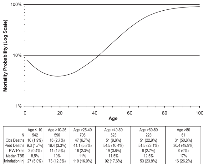
FIGURE 4. Predicted mortality probability from the logistic model of Equation 3 developed with inclusion of fungal information as FWI. The curve has FWI set to “no,” TBS set to 45%, FTBS set to 30%, inhalation injury set to absent, and age points varying across the abscissa. The variables other than age must be held constant over the full range of age, to see only the effect of age in the predicted curve. Entries below the plot represent actual patient data in age groups chosen to represent various parts of the curve. Obs, observed deaths (mortality). Pred, predicted deaths (mortality); pred deaths as the sum of the probabilities calculated with Equation 3 (and actual patient data). Obs and pred mortality are in good agreement across age groups. Age is in years. TBS and FTBS are in percentage body surface area.
