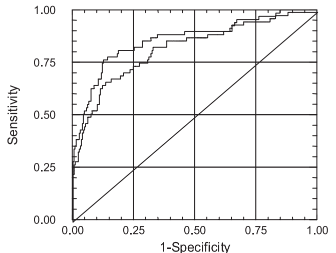
FIGURE 5. Receiver operator characteristic (ROC) curves comparing the ability of the mortality model including FWI as an independent variable (Equation 3) and the model without fungal information (Equation 2) to discriminate between observed survival and nonsurvival. For this comparison and these curves, the 2 models (each developed in all the patients) were applied only to the 298 patients with TBS >30\% – 60\% . The area under the curve (AUC) from application of Equation 3 (AUC = 0.867) was significantly greater ( P = 0.005 ) than that from application of Equation 2 (AUC = 0.826). The straight diagonal line would indicate no discrimination (AUC = 0.5).
