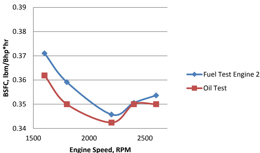
Figure 15: 400hr Engine Brake Specific Fuel Consumption, JP-8, 77F Air, 86F Fuel
