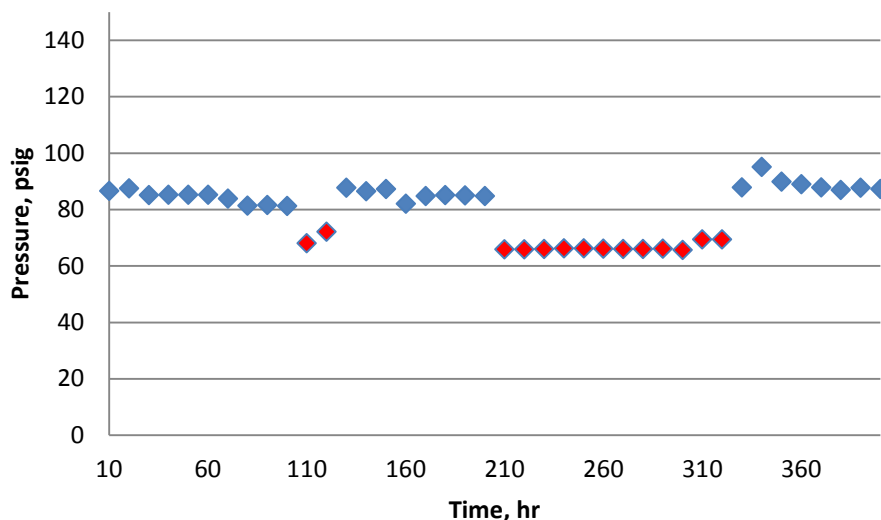
Figure 22: Oil Test Oil Pressure, JP-8, Low Viscosity Oil, 120F Air, 175F Fuel, 400hr, Peak Torque Sub-cycle 9
