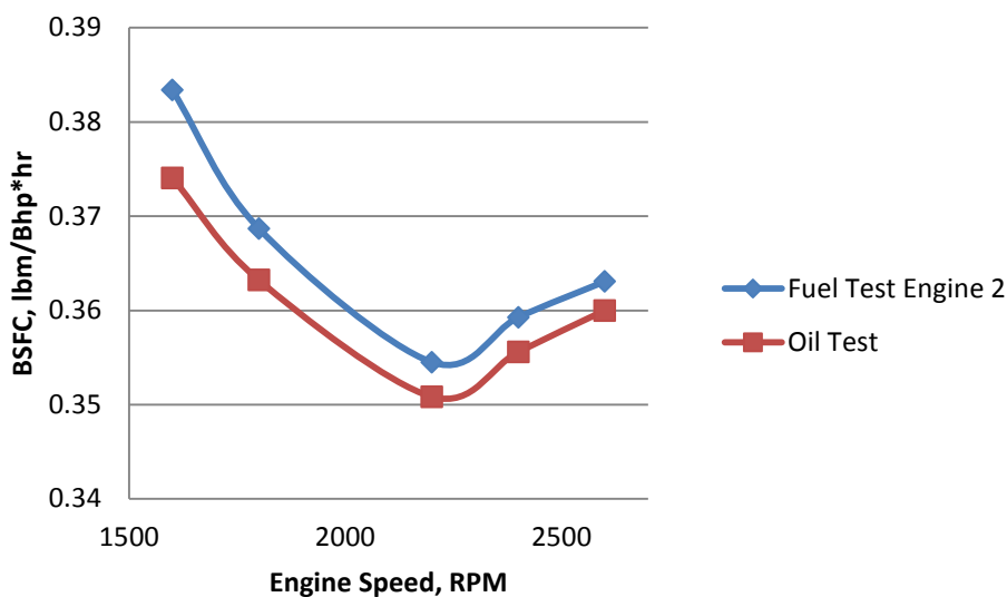
Figure 16: 400hr Engine Brake Specific Fuel Consumption, JP-8, 120F Air, 175F Fuel
