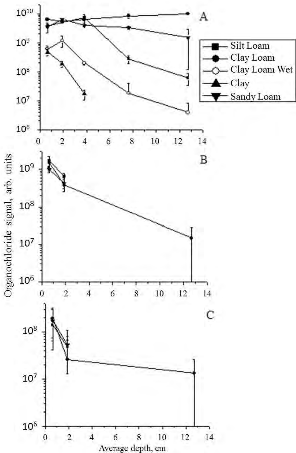
Figure 19. Chlorinated Organic Signal from Soil Headspace (See notes under Figure 18.)
