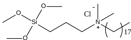
Figure 37. [3-(Trimethoxysilyl)propyl]octadecyldimethylammonium Chloride (Quat)
