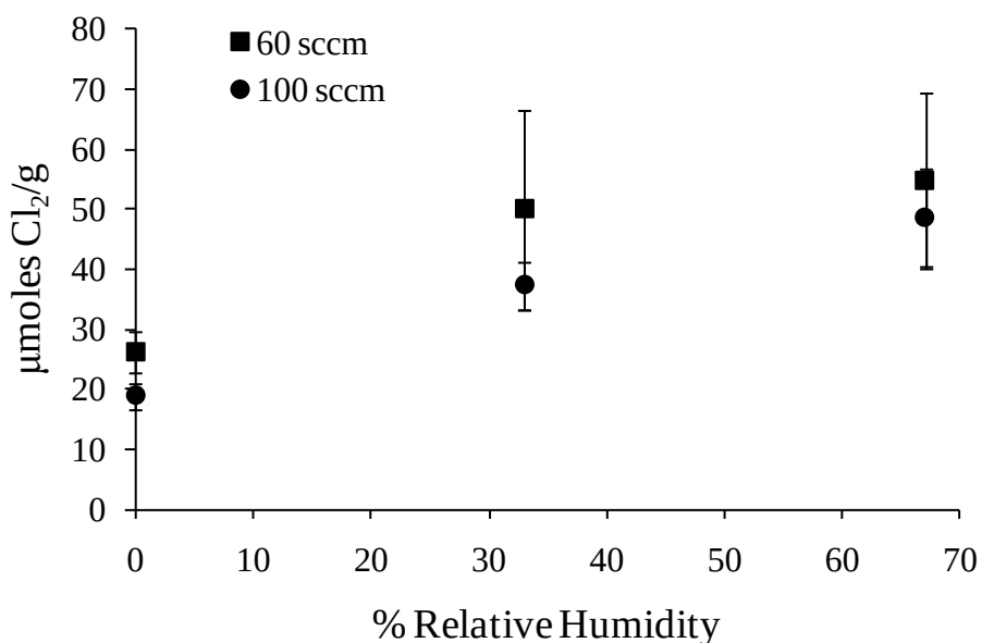
Figure 5. Normalized Uptake of \text{Cl}_2 on Silt Loam as a Function of Humidity \text{Cl}_2 Deposition Was Calculated by Equation (1) to an Exposure of 5 \mu\text{mol} \text{Cl}_2 . Measurements Were Made at 333-ppm \text{Cl}_2 Concentration and the Column Flow Rate Indicated in the Figure Legend; Error Bars Represent the Standard Deviation of the Averaged Measurements.
