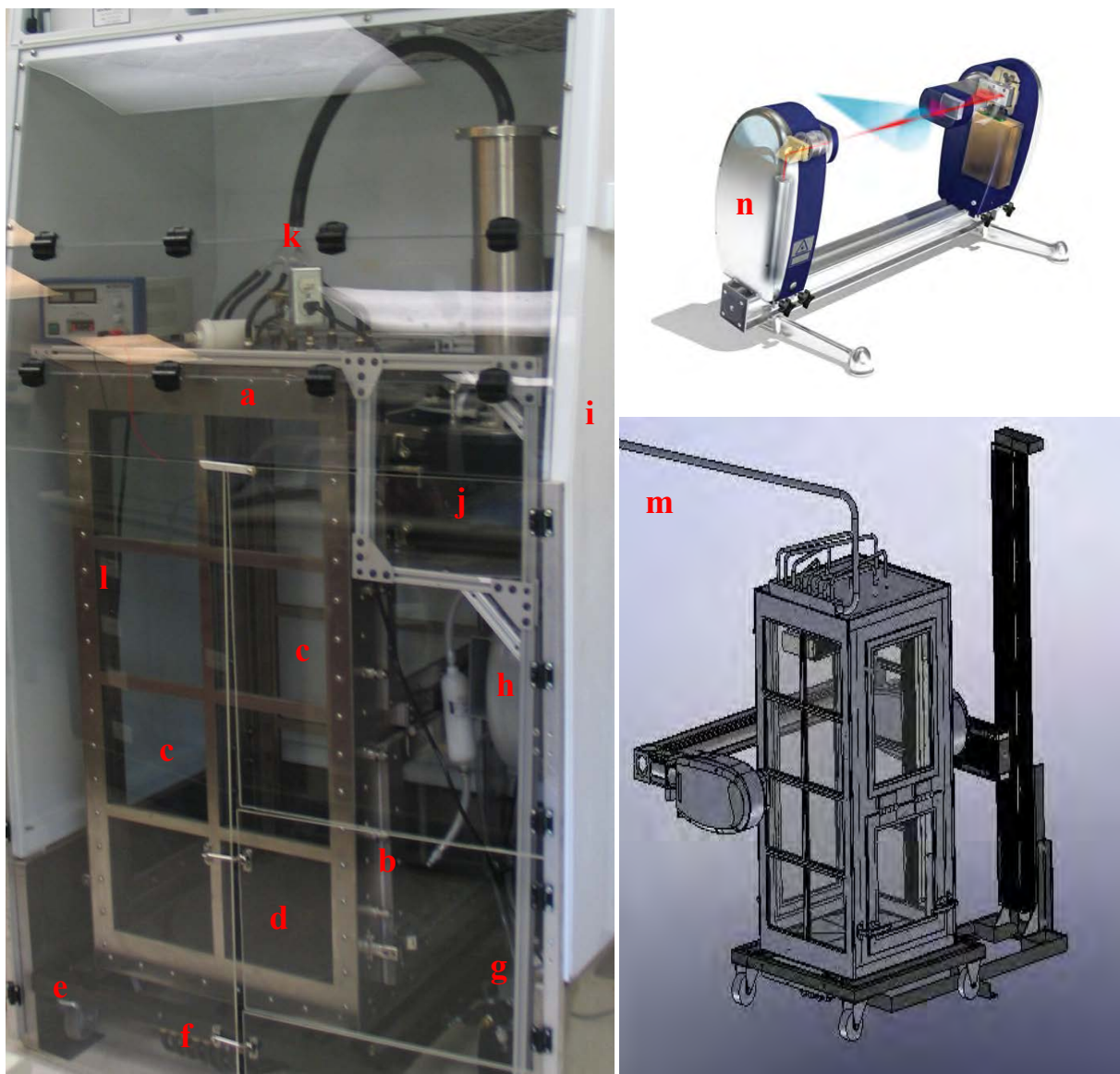
Figure 89. Biological Aerosol Dispersing System (BDS): (a) Chamber (b) Sample Access Door, (c) Optically Clear Glass Panels, (d) Rotating Table, (e) Rolling Cart, (f) Air Exit Manifold, (g) Air Compressor, (h) Air Buffer Tank, (i) Type I Biological Safety Cabinet, (j) Pitt-3 Powdered Aerosol Dispenser, (k) Six-Way Diffuser, (l) Large Access Door, (m) Biological Dispersing System, (n) Malvern Spraytec
