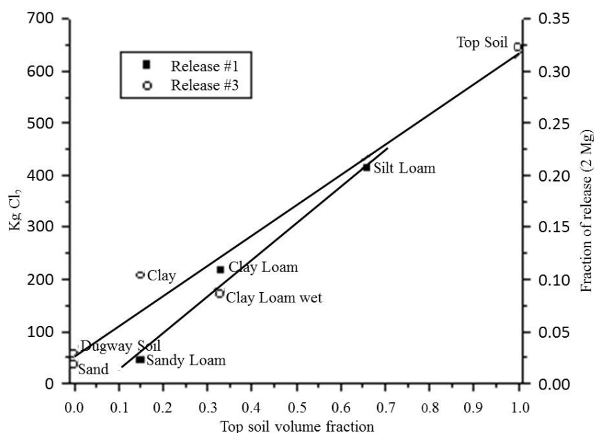
Figure 25. Interpolated Cl 2 Deposition within 20 m from Release Values calculated from chloride concentrations as described in the text. This calculation is based on a Cl 2 penetration depth of 1.27 cm.
