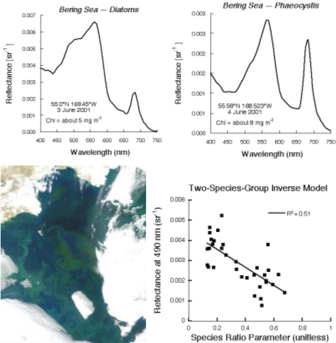
1. Reflectance as measured with a Satlantic Hyperspectral Radiometer Buoy in the Bering Sea during June 2001. During deployment, the radiance sensors are 0.65m below the surface, so the measurement is Lu(\lambda, 0.65\text{m})/Ed(\lambda, 0^+) ( \text{sr}^{-1} ), plotted here as a function of wavelength, \lambda . Note the different scales for diatoms (upper left) vs. Phaeocystis (upper right); the diatom bloom is brighter (reflectance is more than two-fold greater). These two water types probably correspond to the swirls of light green and dark green water in a SeaWiFS image taken the same week (lower left: an image of blooms in the Bering Sea provided by the SeaWiFS Project, NASA's Goddard Space Flight Center, and ORBIMAGE). A new inverse model of ocean color as influenced by diatoms vs Phaeocystis (Huot, Ciotti, and Cullen) yields a species ratio parameter for each of 33 reflectance spectra from the cruise (0 = all diatoms, 1.0 = all Phaeocystis). Preliminary results (a plot of reflectance at 490 nm vs the species ratio parameter; lower right) indicate that the brighter waters (higher reflectance at 490 nm) are dominated by diatoms. This method for discriminating species composition will be evaluated by direct comparison to pigment analysis and results of microscopic examination. Information content of the fluorescence signal will be examined in targeted studies on the interpretation of sun-induced fluorescence.
