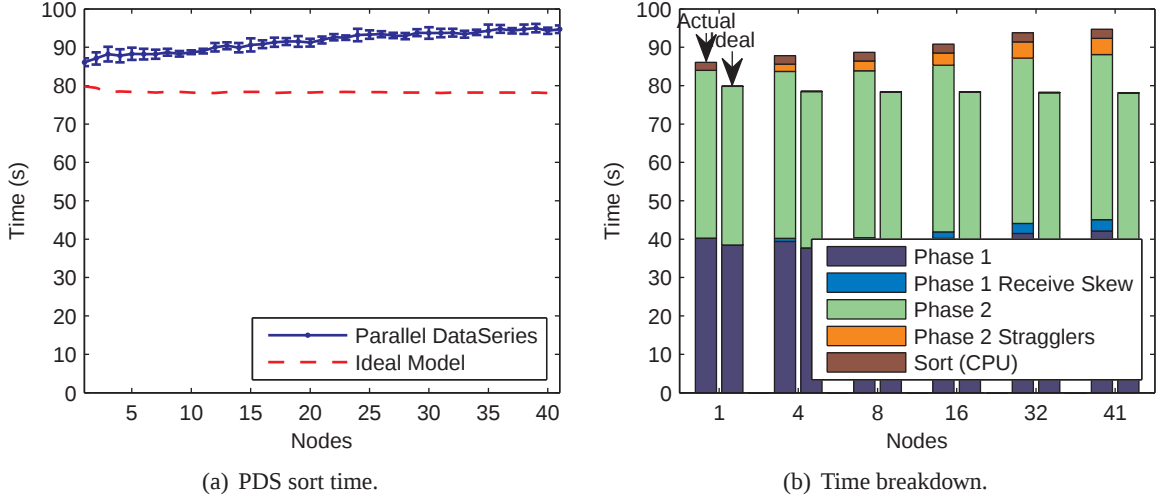
Figure 5: PDS sort performance with a network bottleneck. Using Parallel DataSeries to sort up to 164 GB over 1 Gbps Ethernet, network effects cause completion times to slowly increase from 8 to 21% higher than an ideal prediction that assumes constant 110 MB/s bandwidth into each node. The increase in sort time up to 41 nodes in (a) is only explained partly by the Phase 2 straggler effects as broken down in (b). The longer network shuffle time and skew from Phase 1 is the largest component of the slowly growing parallel sort times.
