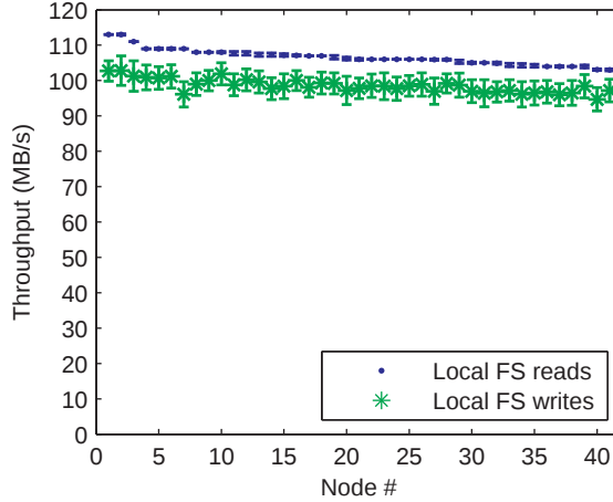
Figure 3: Read and write bandwidth measurements through the XFS filesystems on our C2 cluster. Even after pruning away slower nodes, variance across nodes is significant, and writes are slower than reads.
