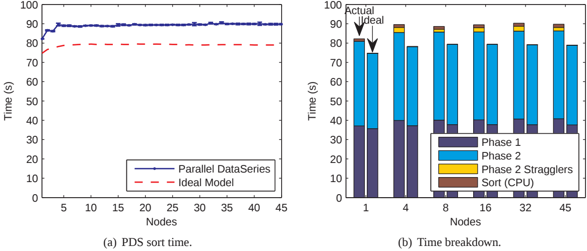
Figure 2: PDS sort performance on a fast network. Using Parallel DataSeries to sort up to 180 GB on a fast 10 Gbps Ethernet, it is possible to achieve within 10 to 14% of the ideal time predicted by our model. PDS scales well up to 45 nodes in (a), sorting 4 GB per node. A breakdown of time in (b) shows that the increases are mostly due to wasted time from nodes in Phase 2 that take longer to complete their assigned work, in addition to a similar Phase 1 increase from disk read skew effects (not explicitly broken out).
