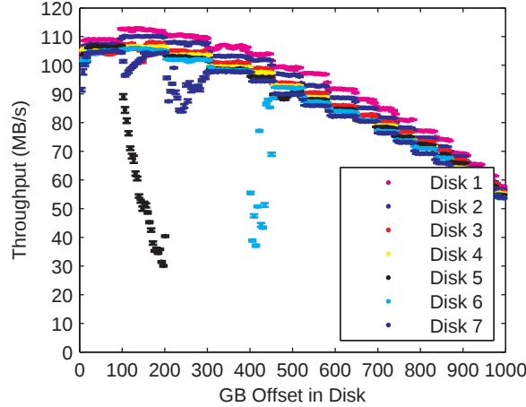
Figure 4: Full-disk streaming read performance. Each of the seven representative disks were selected from a set of twenty-five identical-model 1 TB 2009-era disks. Because of new disk manufacturing methods such as adaptive zoning, disk cluster performance has become increasingly variable, creating a heterogeneous environment that complicates efficient job placement strategies.
