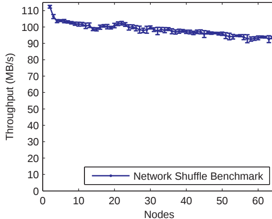
Figure 6: Network shuffle throughput. A separate network shuffle microbenchmark measures the average throughput per node, starting just after initiating all connections and ending when the last bit of data has been received at all the nodes. The quick drop in throughput from two to four nodes, and a gradual slowdown afterwards, confirms that the data shuffle is not effectively using the full link capacity of the network.
