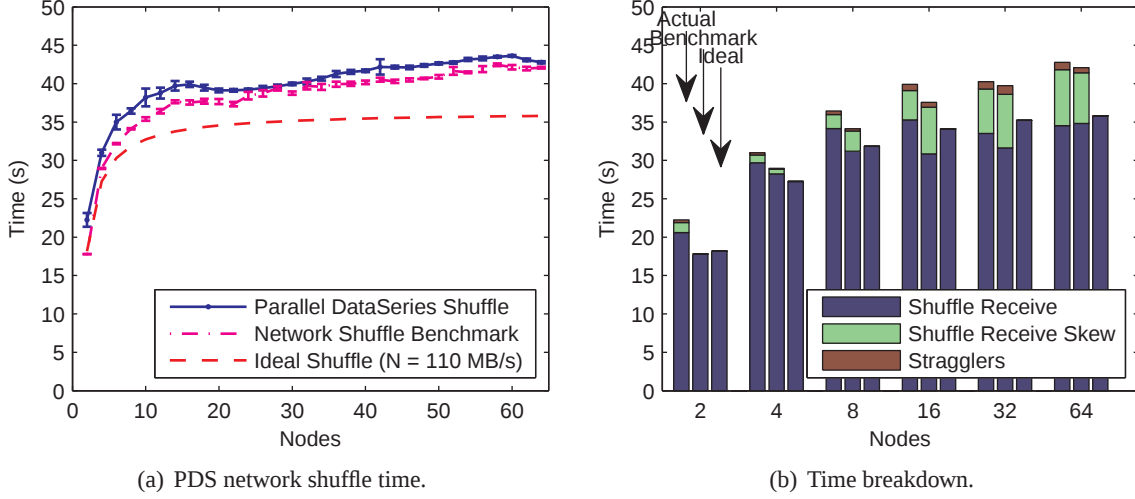
Figure 8: PDS network shuffle performance over 1 Gbps Ethernet. By focusing on just the PDS network shuffle, increases in the completion times are more than the model predicts, mostly because of network slowdown effects. The measured PDS network shuffle times in (a) are slower than the ideal shuffle prediction of the model evaluated with 110 MB/s network speeds, but appear much closer to the measured network shuffle microbenchmark results. The time breakdown in (b) confirms that most of the increased PDS network shuffle time includes receive skew, which measures the skew of incoming flow completion times on every node, as well as a general network slowdown effect that also appears in the microbenchmark.
