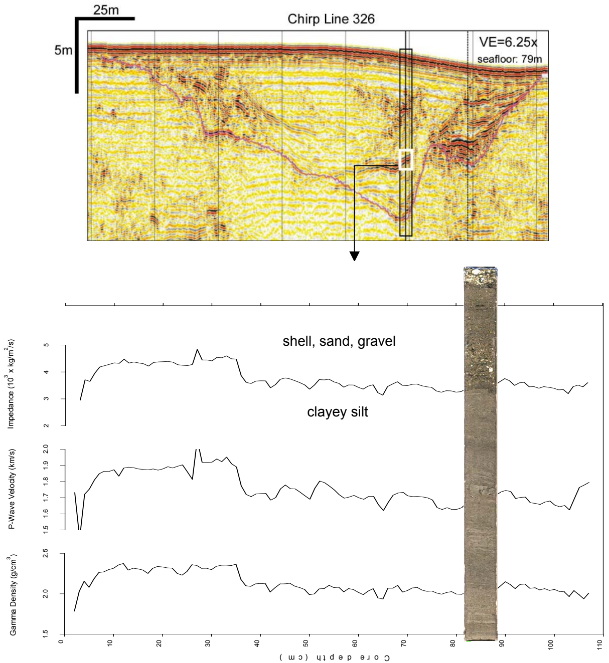
Figure 1. Example of correlated seismic and sediment physical properties data for Geoclutter drillcore Site 2. (Top) Chirp profile showing a buried channel with internal seismic reflectors of variable amplitude. The 13-m section cored during cruise KN-168 is shown (black rectangle). (Bottom) Downcore physical properties and photograph for the core section corresponding to a prominent seismic discontinuity near the channel base (white rectangle). The discontinuity is created by a contrast in acoustic impedance (density x velocity) across a stratal surface formed by the contact of shell-gravel-sand (high impedance) and clayey silt (low impedance). Seismic profile courtesy of UTIG.
