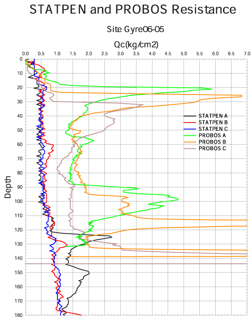
STATPEN and PROBOS Tip Resistance from Gyre 6, Site 5 plotted to same scale. Depth is relative to mudline. Peaks in the PROBOS data at about 30 cm depth are attributed to dilatory behavior of granular layers at that depth.
