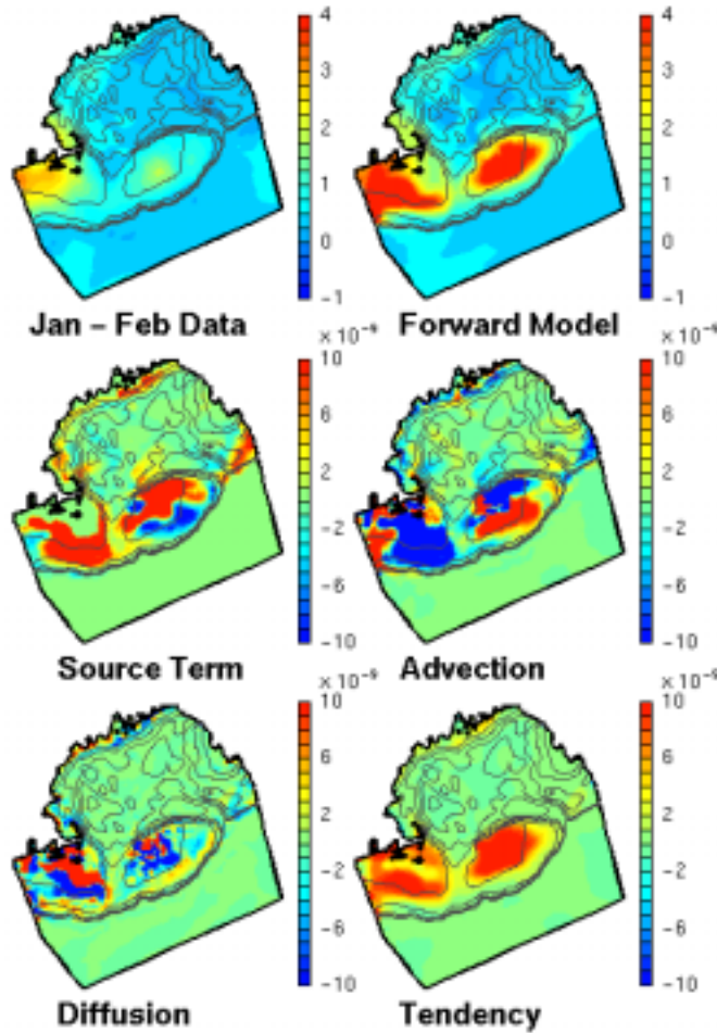
Figure 1. Climatological chlorophyll-a distributions for (a) January-February, and (b) March-April. Note that panel (b) is labeled “Forward Model” because the predictions match the observations so closely. Results of the assimilation procedure and associated sensitivity experiments are also shown: (c) the source term R(x,y) , (d) the advective flux divergence, (e) the diffusive flux divergence, and (f) the overall tendency. Panels (d) through (f) are time-averaged over the 60-day forward simulation.
