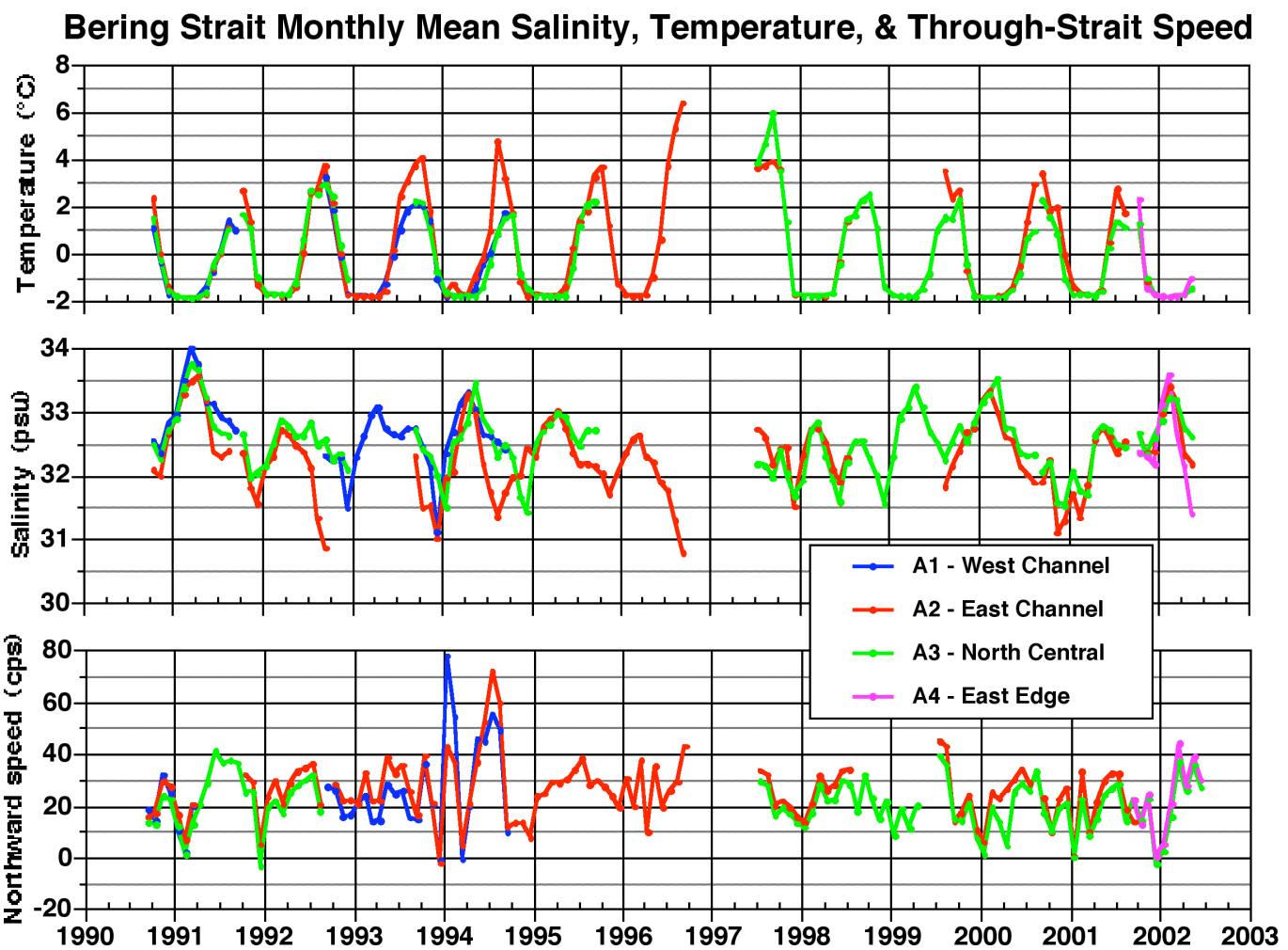
Figure 1: Monthly mean temperature (top), salinity (middle), and throughflow speed (lower) in Bering Strait during 1990-2002. Moorings A1 and A2 respectively measure the middle of the western and eastern channels; A3, located just north of the center of strait, shows characteristics of both channels; and A4 represents the easternmost part of the strait, where a coastal jet is sometimes found.
