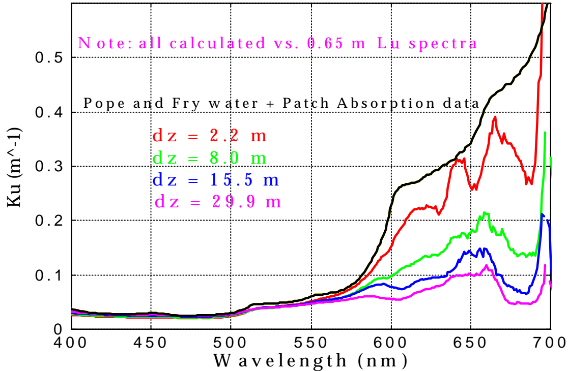
Figure 1. Ku spectra showing the effects of Raman scattering > 520 nm and chlorophyll a fluorescence at 685 nm. See text for discussion.
