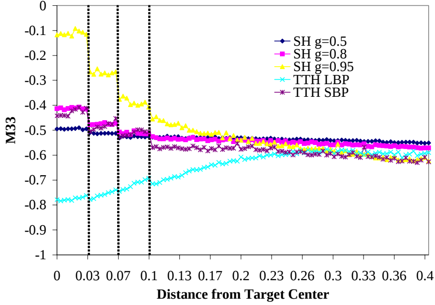
Fig. 3 Same as Fig. 2 except for the element M_{33} . Note the separation in the continuum by g value and the fact that for the high g value (0.95) the effect of the target is seen all the way out to 0.26.
