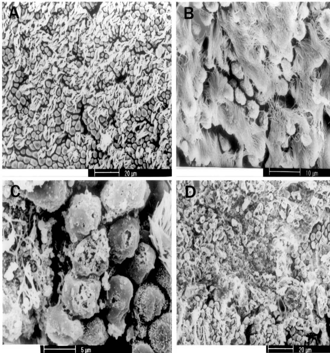
Fig. 4. SEM of rat tracheas at 24 h after injury. (A) Control shows normal tracheal epithelium with both ciliated and non-ciliated cells, \times 800 . (B) Burn only. Group shows some ciliary matting, \times 2000 . (C) Combined smoke and burn. Trachea reveals cellular erosion, \times 4000 . (D) Smoke only. Cellular erosion and pseudomembrane formation (arrow) observed, \times 800 .
